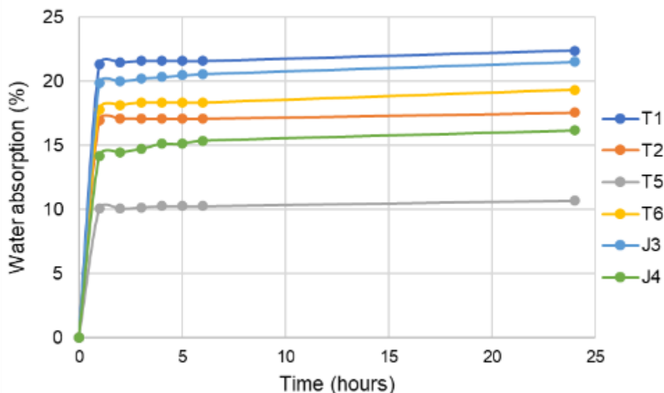
Figure 3. 31. Water absorption of bricks fired at 850 °C with time
