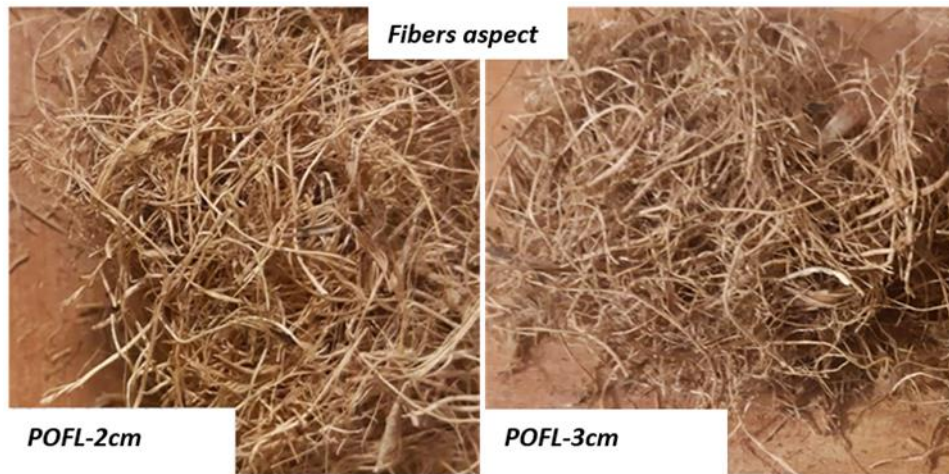
Figure 4. 13. POLF fiber of lengths G-2cm and G-3cm
