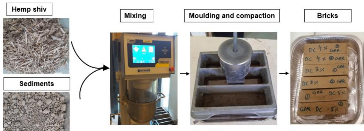
Figure 5. 24. Manufacturing of earth bricks with DK and GAR sediments.
