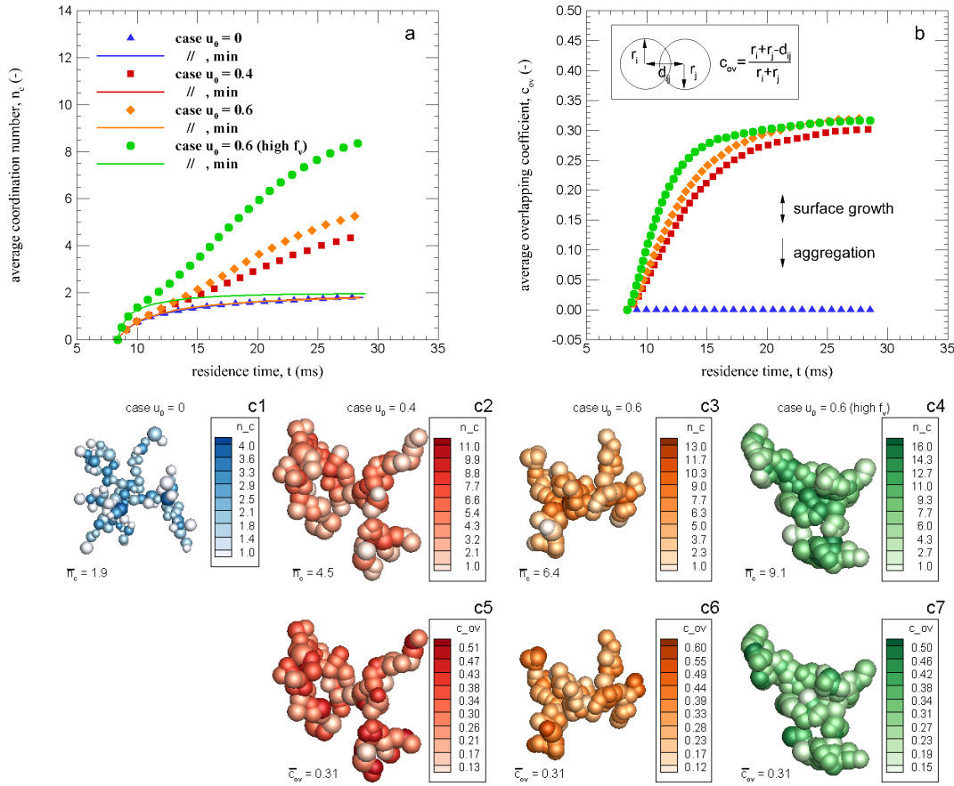
Figure 5.5: Time evolution of the average overlapping coefficient and coordination number. Continuous lines correspond to the minimum coordination number \bar{n}_{c,min} for each case. Examples of aggregates highlighting (by the color bar) the local coordination number (Figs. c1 - c4), and average overlapping coefficient per primary particle (Figs. c5 - c7).
