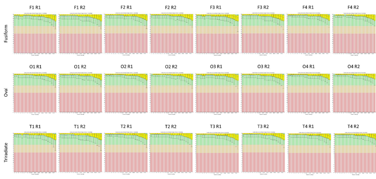
Figure 67: FastQC report depicting per base sequence quality for the 4 biological replicates of the respective enriched cultures for either the fusiform, triradiate or oval morphotype.
