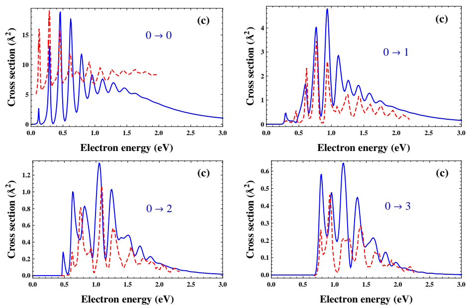
Figure 3.11: Calculated electron-NO resonant cross sections (solid line) compared with the experimental data of Allan (dashed line) [61].
