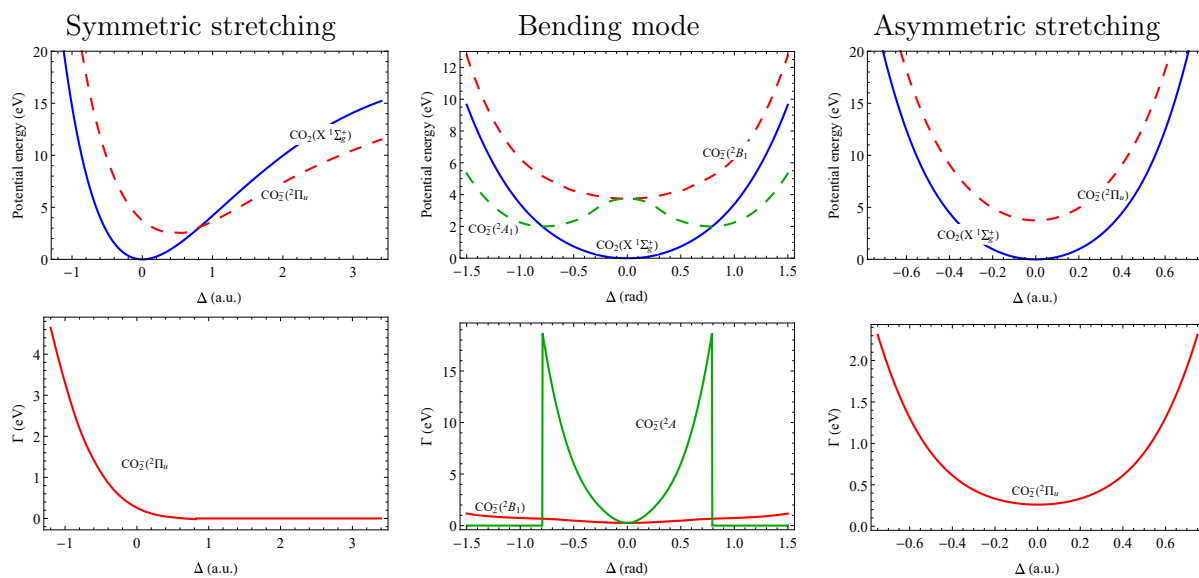
Figure 3.32: Upper panels: Potential energy curves for the electronic ground electronic state X^1\Sigma_g^+ of \text{CO}_2 (full-blue line) and for the resonant state \text{CO}_2^- (dashed-red and green lines) for the three normal modes symmetric stretching, bending and asymmetric stretching. Lower panels: the corresponding resonance widths. \Delta represents the displacement from the equilibrium geometry.
