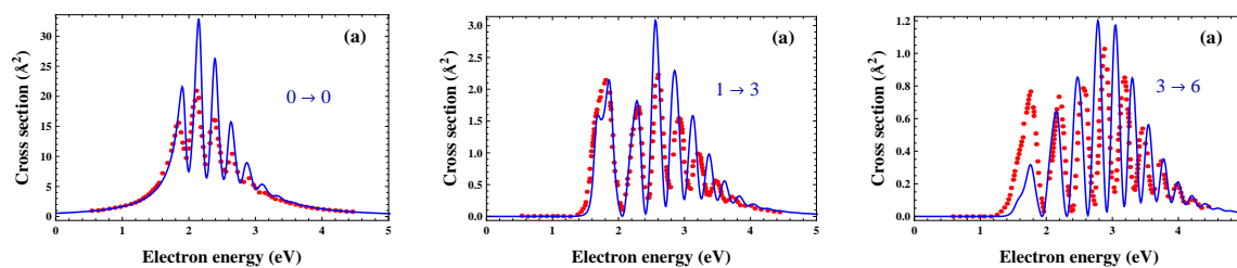
Figure 3.5: Calculated electron- \text{N}_2 resonant cross section (solid line) compared with the results of Dubé and Herzberg [22] (full circle).
