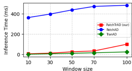
Fig. 3. Inference-time Computation based on SWaT Dataset configuration for various window sizes, with a batch size of 128.
