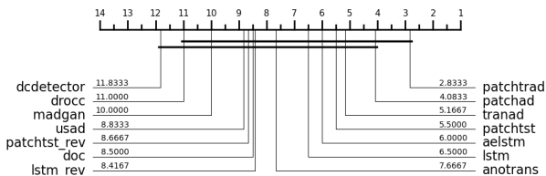
Fig. 2. Critical difference diagrams for AUC scores using the post-hoc Nemenyi test with \alpha = 5\% , where better-ranked methods appear on the upper right.
