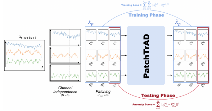
Fig. 1. PatchTrAD Overview.
