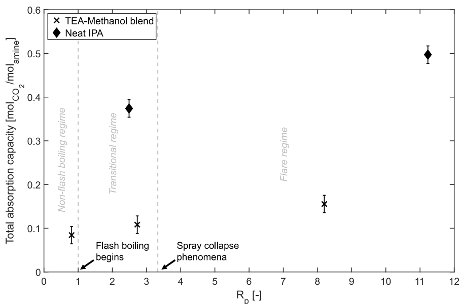
Fig. 19. Total absorption capacity vs R_p for the tested TEA-methanol and neat IPA solvents.
