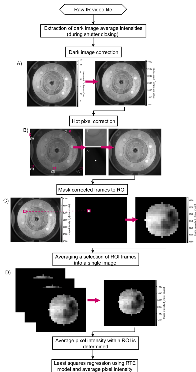
Fig. 5. Image processing methodology flow chart for correcting raw IR frames, masking procedure with ROI, averaging pixel intensities in ROI, and least squares model fitting with RTE equation. (A) Subtraction of average image counts during shutter closing (non-uniformity correction). (B) Correcting saturated pixels in red squares via replacing them by the average of neighbouring pixels. (C) Corrected video file with ROI highlighted in red box. (D) Masked frames are averaged into a single image which is then used for model fitting.
