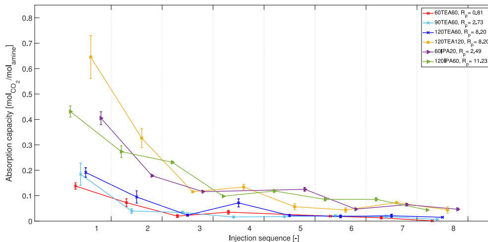
Fig. 17. Absorption capacity vs injection sequence for each temperature condition and amine tested. Error bars represent the expanded standard uncertainties of absorption capacity at each injection sequence.
