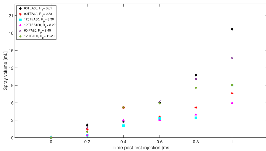
Fig. 9. Estimated spray volume as a function of time, from start to end of injection. The spray volume was estimated from the spray angle and penetration length using a conical shape approximation.
