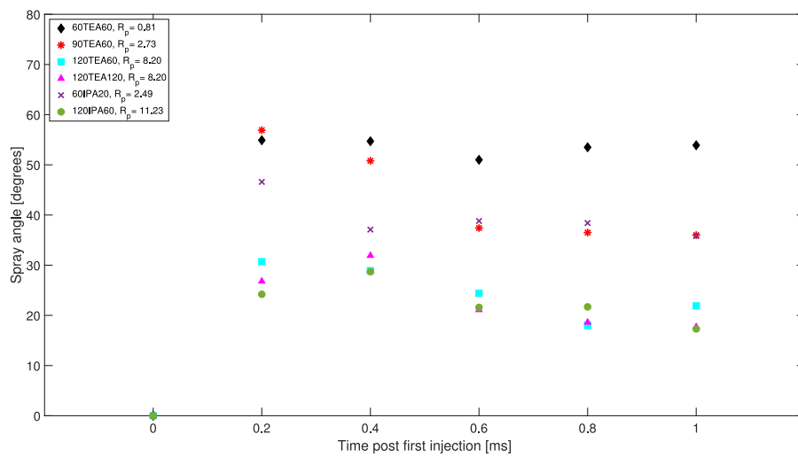
Fig. 8. Spray angle for each tested condition as a function of time.
