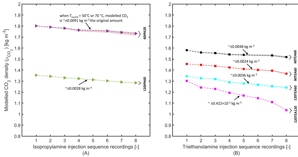
Fig. 14. Temperature sensitivity analysis when only nozzle temperature is raised/decreased by \pm 10^\circ\text{C} for the (A) Isopropylamine data set (B) Triethanolamine data.
