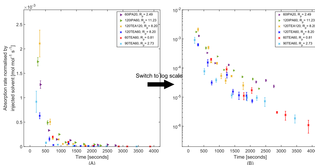
Fig. 18. Absorption rate normalised for injected solvent at each injection sequence vs time. (A) Absorption rate in a linear scale vs time. (B) Absorption rate in log scale vs time. Error bars represent the expanded uncertainties of molar absorption rate at each injection sequence.
