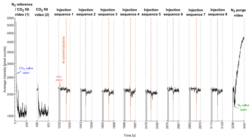
Fig. 10. Non-uniformity corrected (NUC) average signal intensity within the masked ROI vs time for all recordings under the condition 120TEA60 ( T_{\text{solvent}} = 120^{\circ}\text{C} , T_{\text{CO}_2} = 60^{\circ}\text{C} ) in order of experimental procedure from left to right. Injection of solvent in each recording is indicated by vertical orange dashed lines. (For interpretation of the references to colour in this figure legend, the reader is referred to the web version of this article.)
