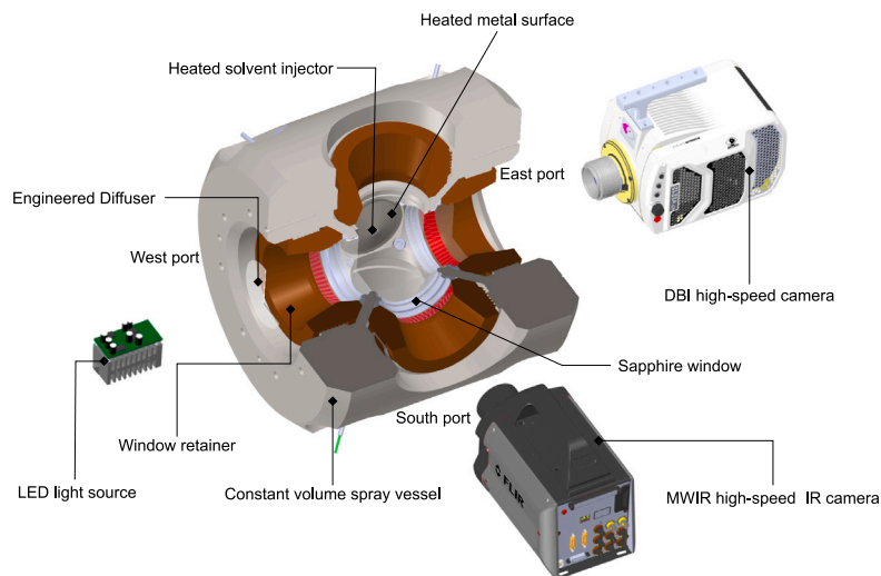
Fig. 1. Schematic of experimental design displaying position of 532 nm LED, MWIR camera, and high-speed camera relative to the constant volume spray vessel and injector.
