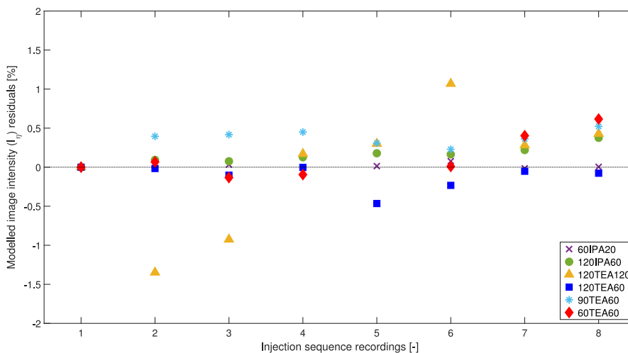
Fig. 12. Image intensity residuals of the model post regression fitting with experimental signal intensities for all tested conditions.
