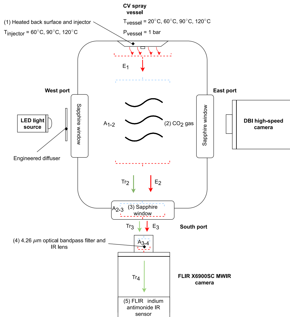
Fig. 4. Heat transfer diagram starting from the heated metal surface/injector towards the MWIR camera. Each absorbing/emitting component in the rig is numbered (1–5). Labels “A” indicate points where IR absorption takes place (e.g. A_{1-2} indicates absorption of incident radiation coming from the injector by the \text{CO}_2 gas). Labels “E” indicate IR emission sources (e.g. E_2 indicates emission from the \text{CO}_2 gas). Labels “Tr” indicate transmitted IR radiation (e.g. T_{r2} represents IR radiation transmitted through the \text{CO}_2 gas).
