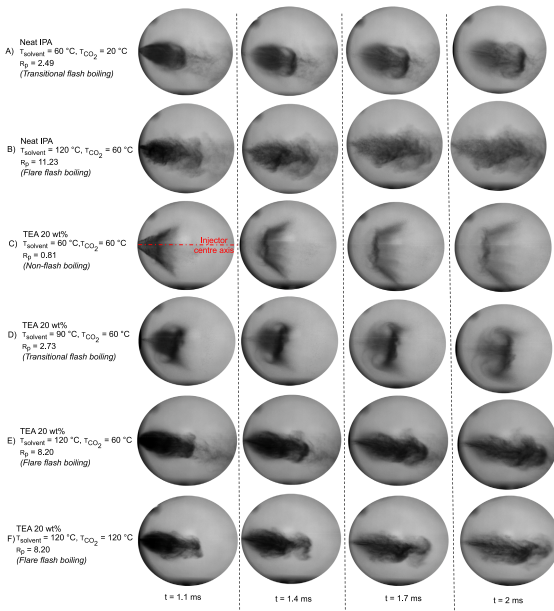
Fig. 6. DBI snapshots of spray evolution after injection for all tested conditions and solvents.
