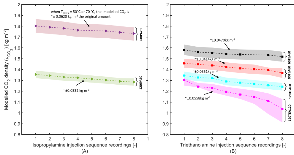
Fig. 15. Temperature sensitivity analysis when only gas temperature is raised/decreased by \pm 10^\circ\text{C} for the (A) Isopropylamine data set (B) Triethanolamine data.
