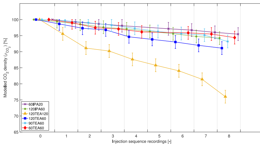
Fig. 13. Model predicted CO 2 values from the beginning the test procedure to the final injection sequence recording.
