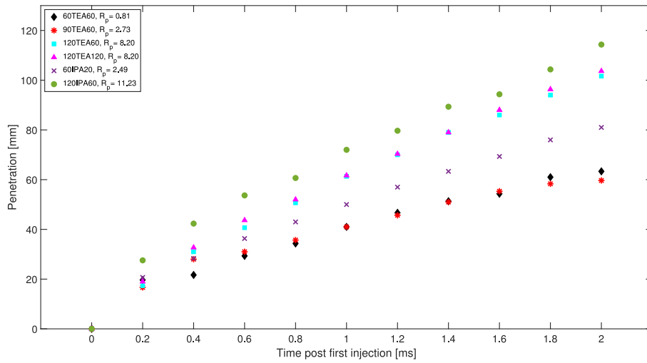
Fig. 7. Spray penetration for each tested condition as a function of time.
