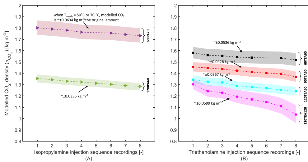
Fig. 16. Temperature sensitivity analysis when both nozzle and gas temperature is raised/decreased by \pm 10^\circ\text{C} for the (A) Isopropylamine data set (B) Triethanolamine data.
