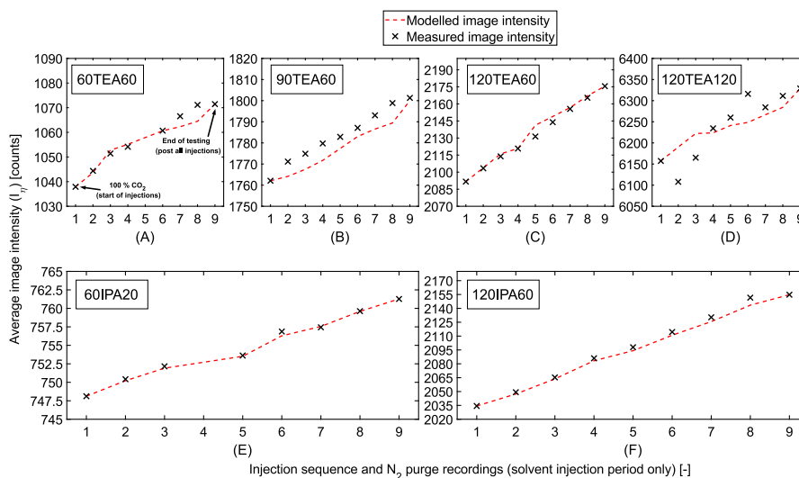
Fig. 11. Measured and modelled image intensity vs injection sequence and \text{N}_2 purge IR recordings for conditions (A) T_{\text{TEA}} = 60^{\circ}\text{C} , T_{\text{CO}_2} = 60^{\circ}\text{C} , (B) T_{\text{TEA}} = 90^{\circ}\text{C} , T_{\text{CO}_2} = 60^{\circ}\text{C} , (C) T_{\text{TEA}} = 120^{\circ}\text{C} , T_{\text{CO}_2} = 60^{\circ}\text{C} , (D) T_{\text{TEA}} = 120^{\circ}\text{C} , T_{\text{CO}_2} = 120^{\circ}\text{C} , (E) T_{\text{IPA}} = 60^{\circ}\text{C} , T_{\text{CO}_2} = 60^{\circ}\text{C} , (F) T_{\text{IPA}} = 120^{\circ}\text{C} , T_{\text{CO}_2} = 60^{\circ}\text{C} .
