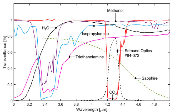
Fig. 2. Spectral chart displaying transmissivity of IR radiation through the species/components present within the experimental setup.
