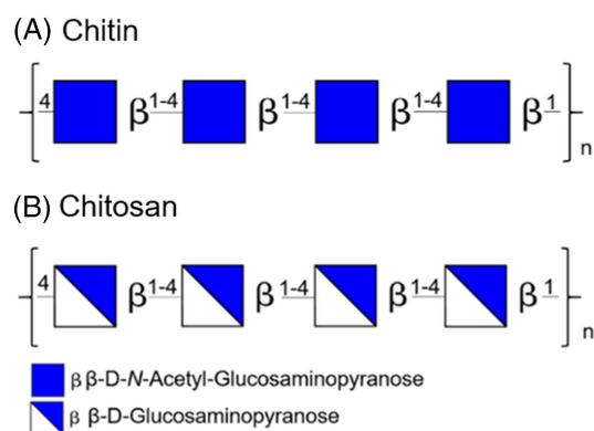
FIGURE 3 Structure of chitin found in the cell wall of fungi (Hou et al., 2021). Chitosan is a deacetylated form of chitin occurring naturally in Mucoraceae (Aranaz et al., 2021) or obtained chemically by alkali treatments. Monosaccharides are represented according to the SNFG nomenclature (Varki et al., 2015) using the Polys Glycan builder monosaccharides ( https://glycan-builder.cermav.cnrs.fr/ ).
