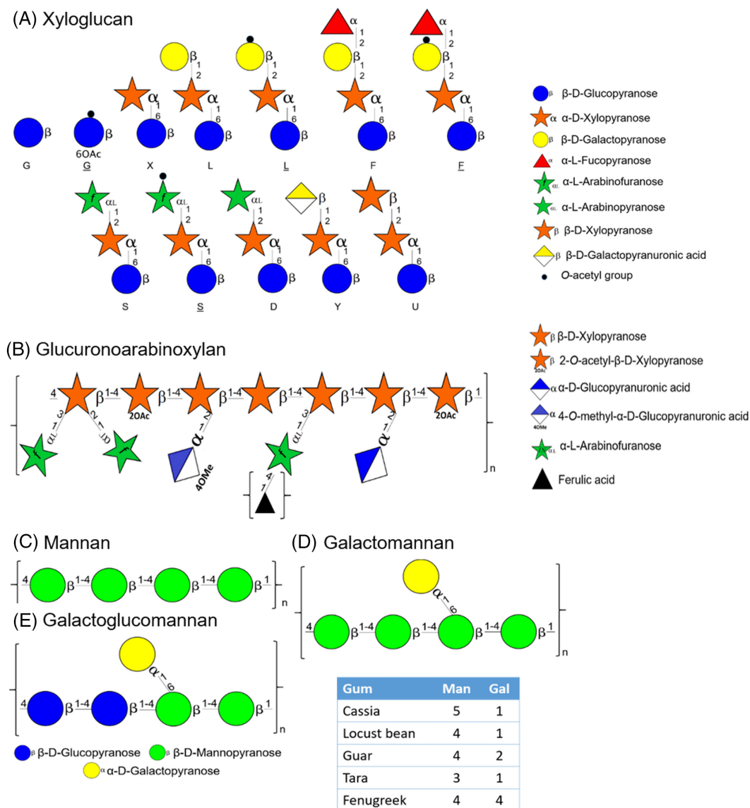
FIGURE 6 Structure of hemicelluloses. Several examples of the diversity of side chains found in xyloglucan depending on the species, organ and tissues (Schultink et al., 2014; Dehors et al., 2019) using the one letter code proposed by Fry et al., (1993). Xylan-type hemicellulose has been described as unbranched xylan backbone, arabinoxylan (AX), glucuronoarabinoxylan (GAX), and 4-O-methyl-GAX (Scheller and Ulvskov, 2010). Ferulic acid is only found in the cell walls of commelinid monocots. Mannan-type hemicellulose can be found as mannan, galactomannan and galactoglucomannan (Scheller and Ulvskov, 2010). Galactomannan gums such as cassia are found in Cassia sp. and Senna sp., locust in Ceratonia siliqua , guar in Cyamopsis sp., tara in Caesalpinia spinosa and fenugreek in Trigonella foenum-graecum seeds (Dhull et al., 2022). Monosaccharides are represented according to the SNFG nomenclature (Varki et al., 2015) using the Polys Glycan builder monosaccharides ( https://glycan-builder.cermav.cnrs.fr/ ).
