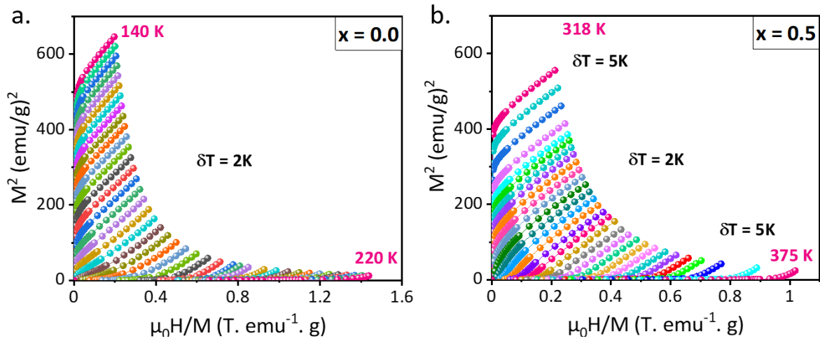
Fig. 6. Arrott plots of for x = 0.0 (a) and x = 0.5 (b) \text{Fe}_{1-x}\text{Cu}_x\text{Cr}_2\text{S}_4 samples at various temperatures.
