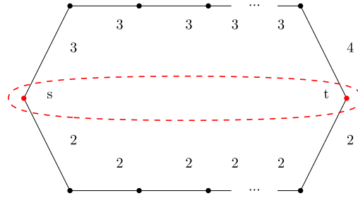
Fig. 5. A graph family admitting an open S^B component for \Delta = 2 (in dashed and red with vertex s as source) and an open \mathcal{T}^B component for \Delta = 2 (in dashed and red with vertex t as sink).
