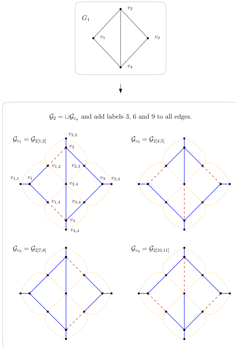
Fig. 7. Example of transformation from a CLIQUE instance graph G_1 to a S^D COMPONENT instance temporal graph \mathcal{G}_2 . For visibility, for all \mathcal{G}_{v_i} , blue full edges correspond to edges with label 3a - 2 , red dashed edges to edges with label 3a - 1 , and orange dotted edges to background edges with label 3a - 1 . Also for visibility, not all background edges are represented.
