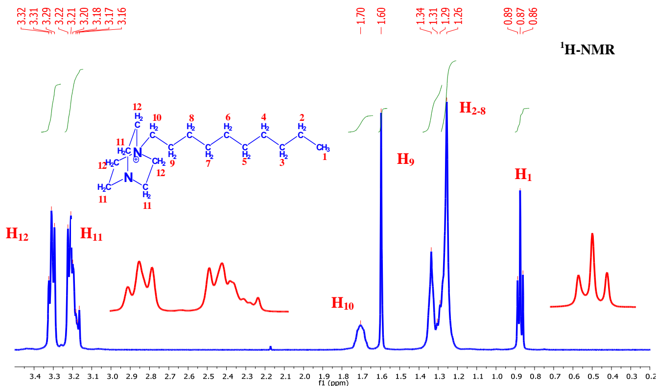
Figure 1. (a) Hydrogen atom labeling and 1 H-NMR spectrum of the DABCO cation.
