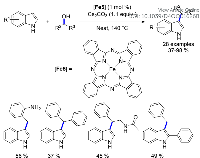
Scheme 83. Alkylation of indoles reported by Piersanti.
