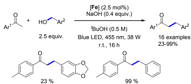
Scheme 109. Alkylation of aryl ketones with benzylic alcohols.
