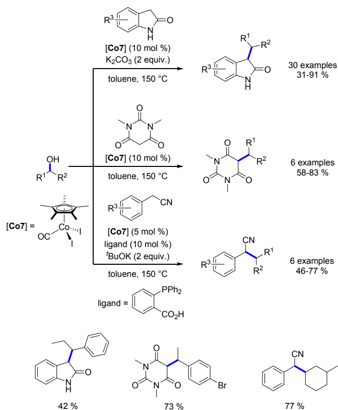
Scheme 98. Alkylation of oxindoles, barbituric acid and nitriles. 1)
