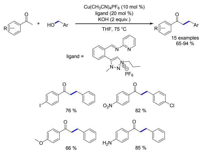
Scheme 105. Copper-catalysed alkylation of ketones.
