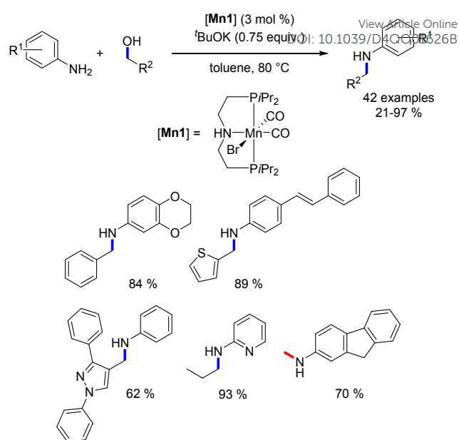
Scheme 6. Manganese-catalysed alkylation of amines.
