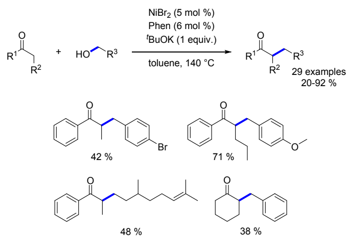
Scheme 100. Alkylation of \alpha -substituted ketones.
