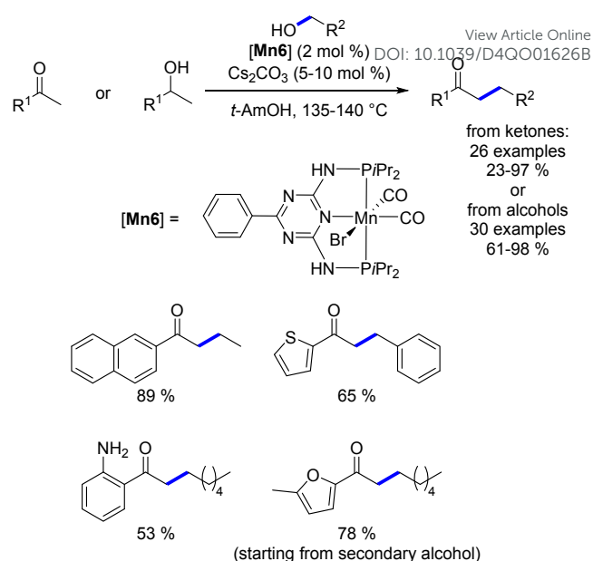
Scheme 66. Synthesis of \alpha -substituted ketones.
