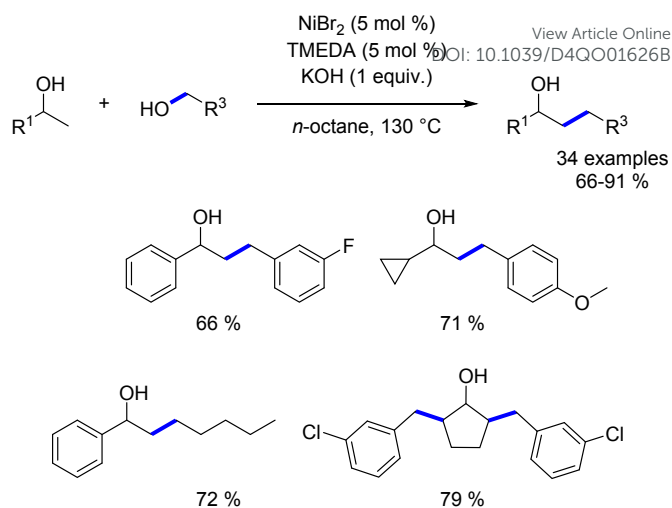
Scheme 102. Nickel-catalysed β-alkylation of alcohols.
