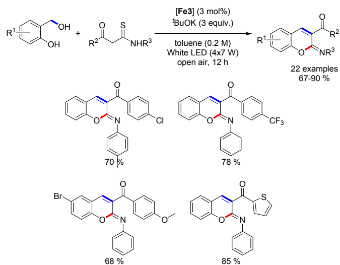
Scheme 107. Synthesis of 2-arylmino-2H-chromenes.
