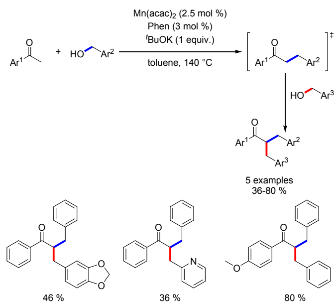
Scheme 72. Two-step one-pot dialkylation of ketones.
