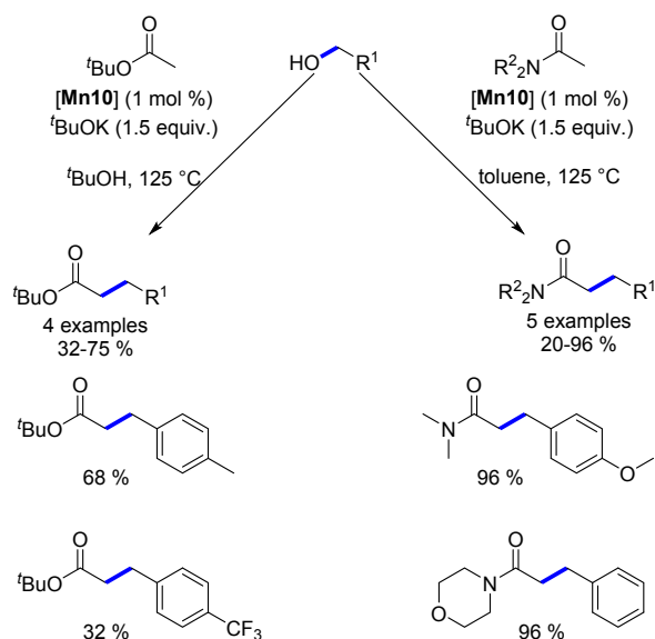
Scheme 58. Milstein's work on the alkylation of amides and esters.
