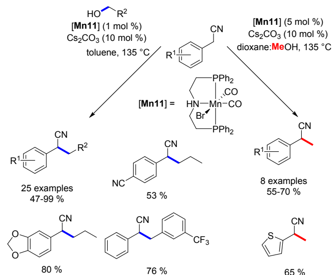
Scheme 59. Alkylation of Nitriles Reported by Rueping.
