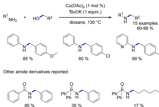
Scheme 49. Copper-catalysed alkylation of anilines and amides derivatives.
