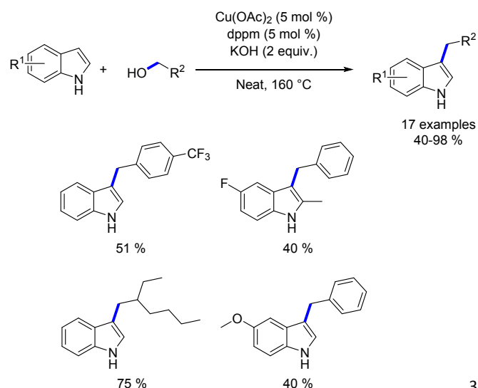
Scheme 104. C3-alkylation of indoles.
