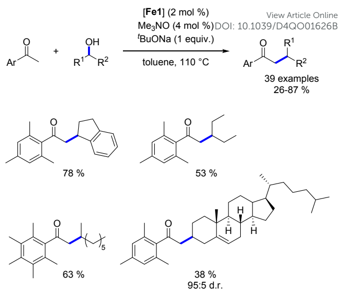
Scheme 87. Alkylation with secondary alcohols.
