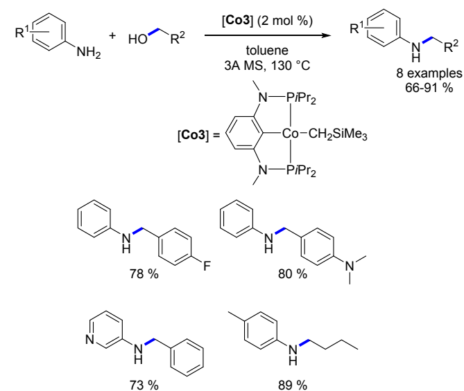
Scheme 35. Base-free alkylation of amines reported by Kirchner.
