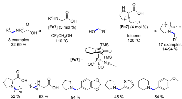
Scheme 23. Alkylation of amino-acids and synthesis of N-substituted cyclic amines.
