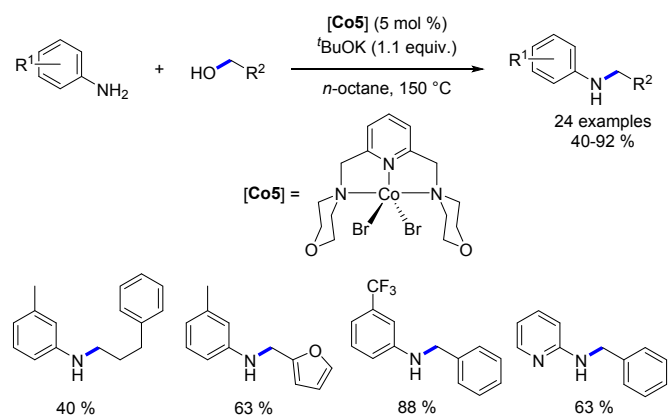
Scheme 39. Cobalt-pincer complex-catalysed alkylation of anilines.
