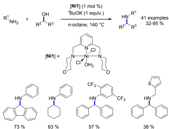
Scheme 45. Alkylation of amines with secondary alcohols reported by Balaraman.
