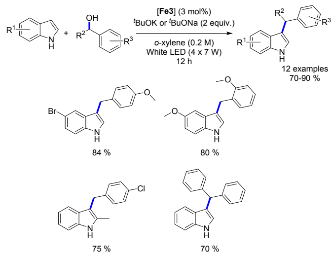
Scheme 108. Alkylation of indoles.
