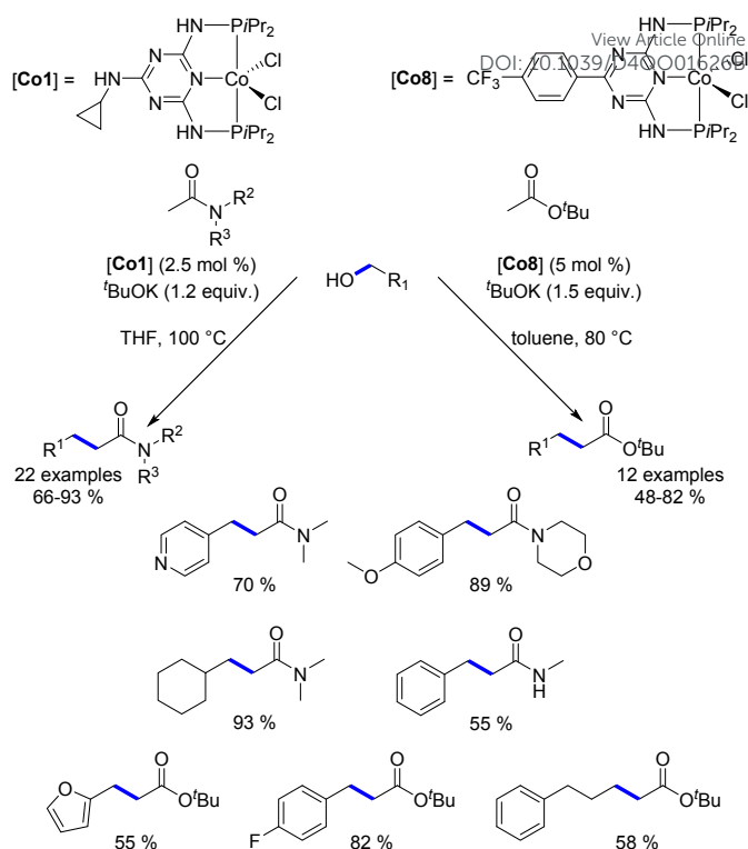
Scheme 90. C-alkylation of amides and esters.
