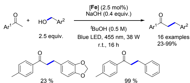
Scheme 109. Alkylation of aryl ketones with benzylic alcohols.
