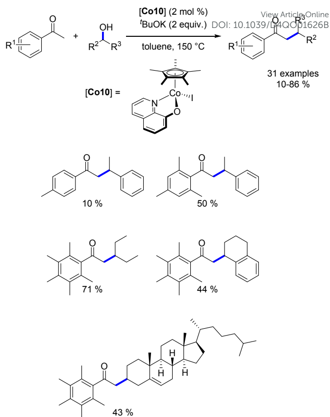
Scheme 97. Alkylation of ketones with secondary alcohols.
