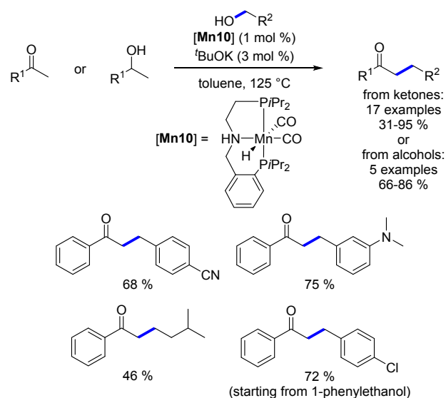
Scheme 57. Alkylation of ketones and secondary alcohols as described by Milstein.
