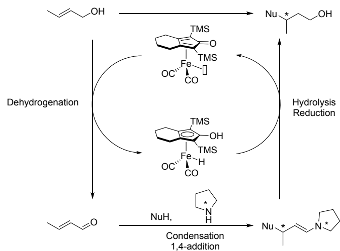
Scheme 75. Dual iron/organocatalysed alkylation of allylic alcohols.
