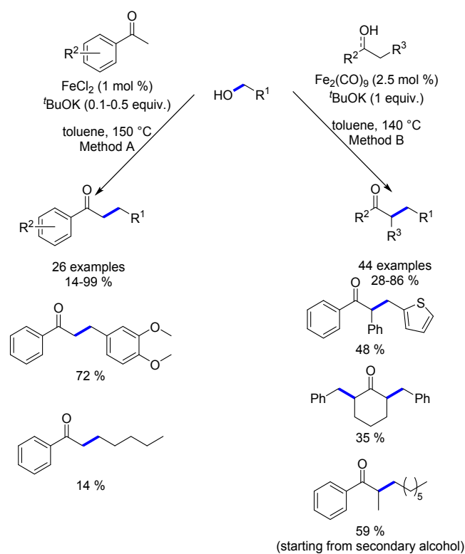
Scheme 88. Synthesis of α-substituted ketones.
