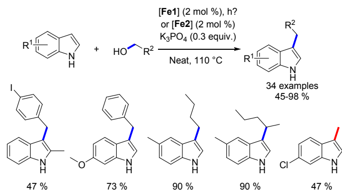
Scheme 82. Alkylation of indoles reported by Renaud.
