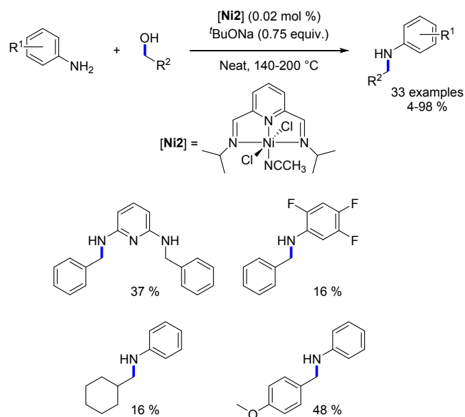
Scheme 46. Alkylation of amines reported by Kumar.
