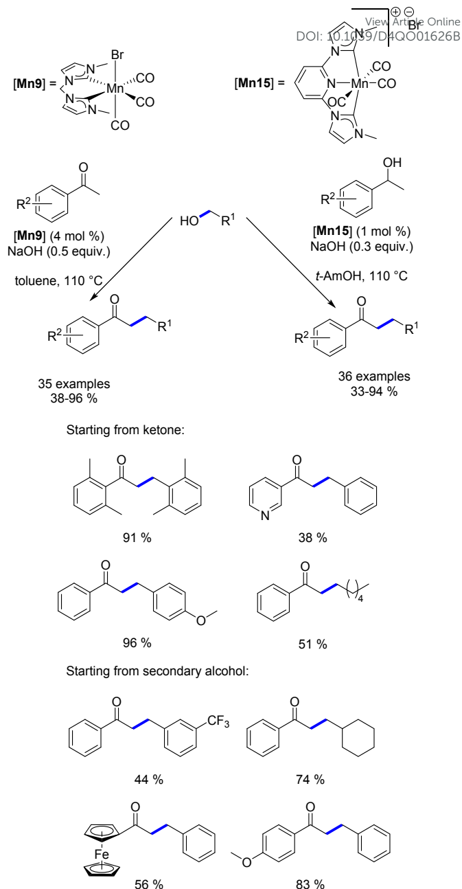
Scheme 73. Synthesis of \alpha -substituted ketones described by Ke.
