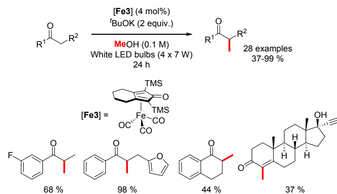
Scheme 106. Methylation of ketones under light irradiation.
