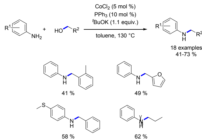
Scheme 37. Cobalt-catalysed alkylation of anilines reported by Balaraman.
