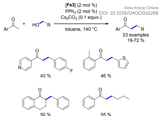
Scheme 79. Alkylation of ketones reported by Darcel.
