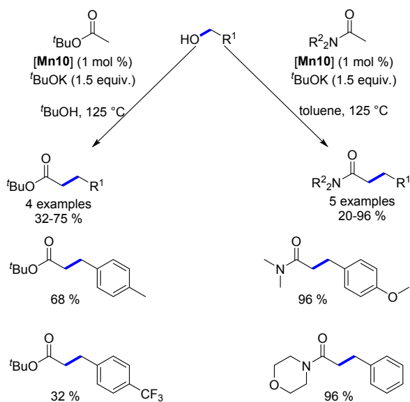
Scheme 58. Milstein's work on the alkylation of amides and esters.
