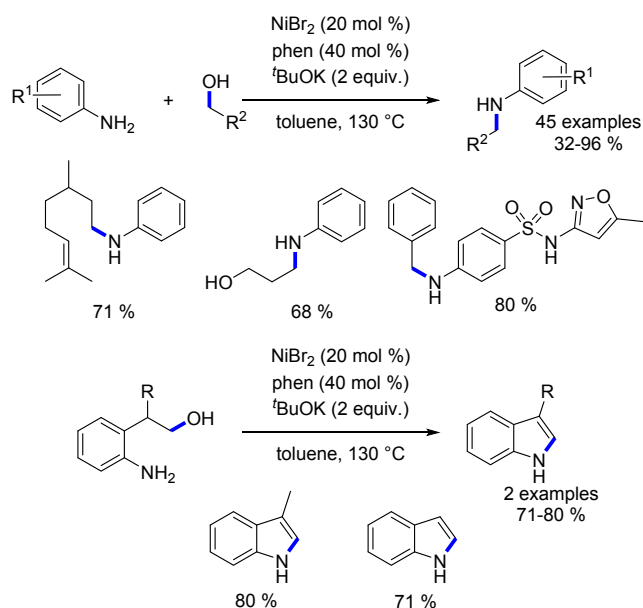
Scheme 43. Alkylation of anilines reported by Banerjee.
