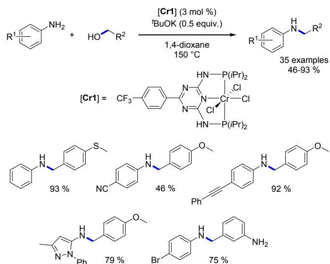
Scheme 54. Chromium-catalysed alkylation of anilines.
