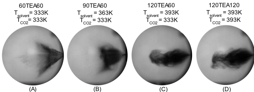
Figure 6. Spray morphology from the POV of the Phantom high-speed camera with image scaling of 0.200 mm/pixel at (A) 333K solvent temperature and vessel temperature (B) 363K solvent temperature and 333K vessel temperature (C) 393K solvent temperature and 333K vessel temperature (D) 393K solvent temperature and vessel temperature.
