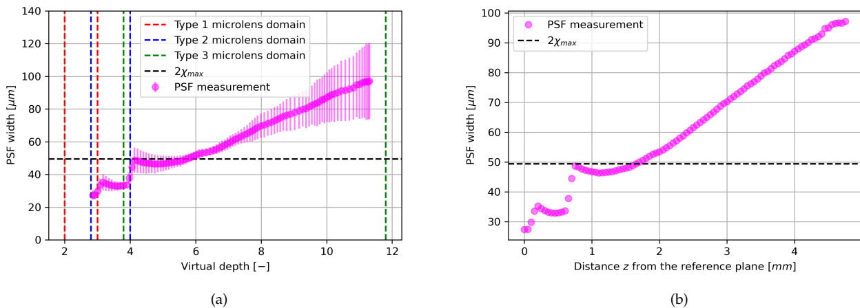
Figure 5. (a) Evolution of the PSF width with the virtual depth v , (b) Evolution of the PSF width with the depth position z in the object space
