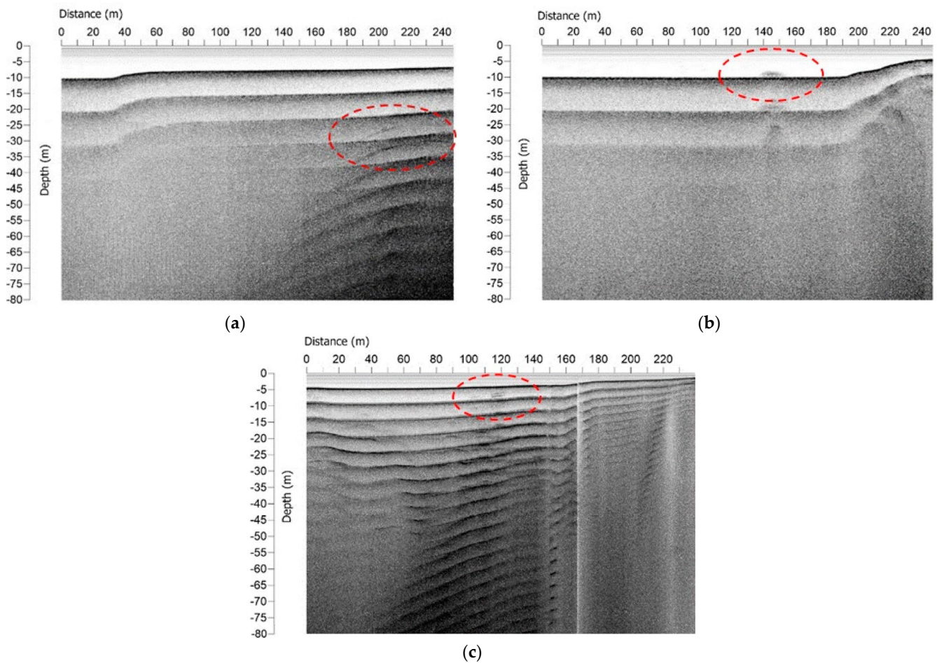
Figure 4. Examples of structures and objects present within the Camastra reservoir: (a) dam weir; (b) boulder or vegetation present on the seabed; (c) bridge connecting two banks of the reservoir.
