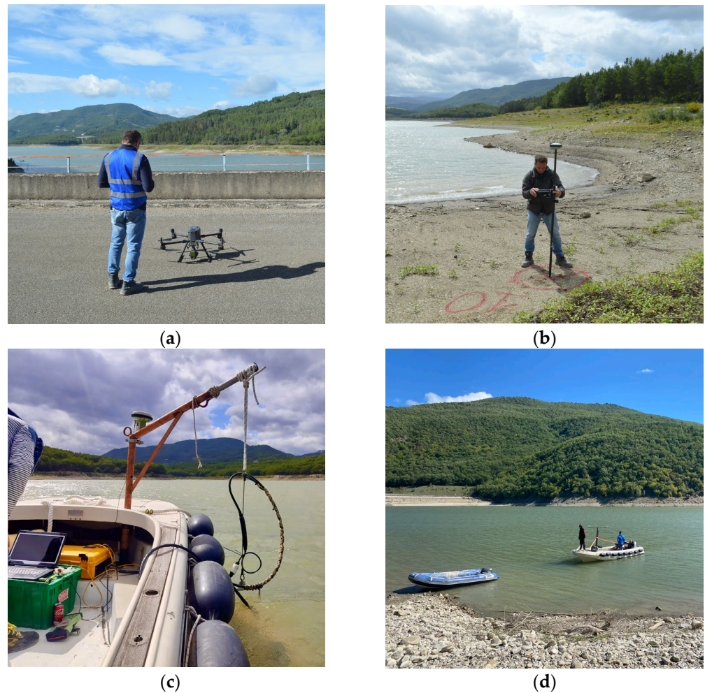
Figure 2. Surveys carried out at the Camastra reservoir: (a) drone survey, (b) GPS survey, (c) and (d) morpho-bathymetric and sub-bottom profiler surveys.
