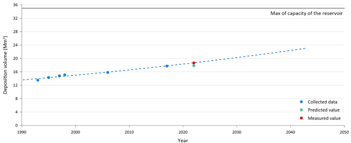
Figure 6. Evolution of the silting phenomenon over the years, forecast with model calculations up to 2022 (green point), and identification of the average value measured following the in situ survey in 2022 (red point), where the collected data are data from previous surveys and the measured value is the value deriving from the 2022 in situ survey.
