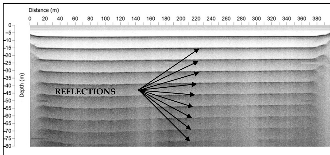
Figure 3. Multiple reflections found in the sub-bottom profiler survey of the Camastra reservoir.
