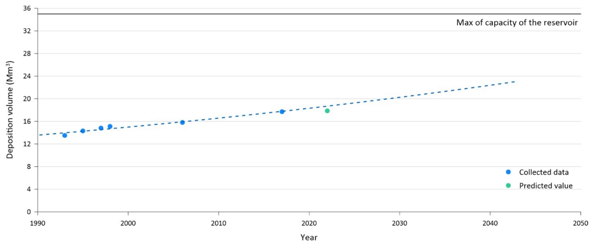
Figure 5. Silting evolution over the years and values forecast with model calculations up to 2022 (green point).
