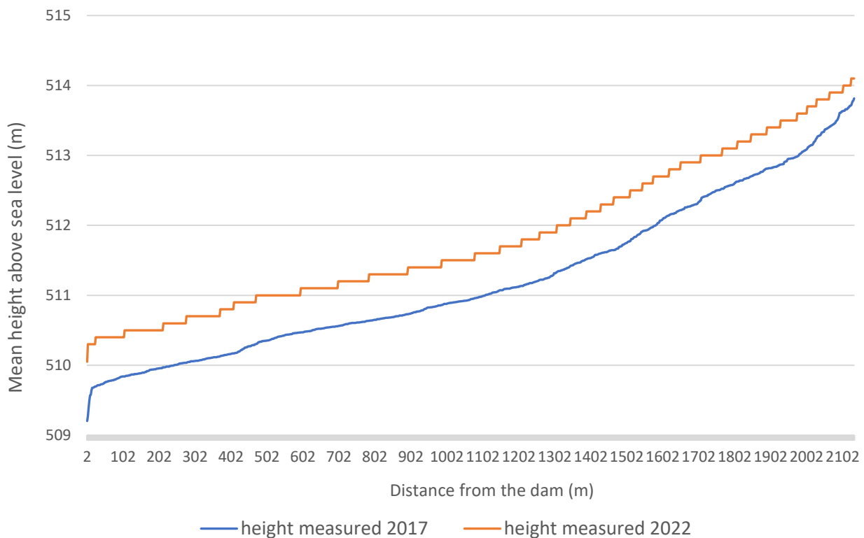
Figure 7. Comparison of seabed elevations measured in the 2017 survey (blue) and 2022 survey (orange).
