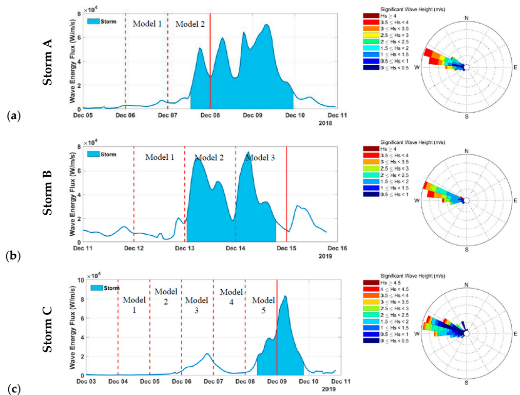
Figure 5. Energy conditions associated to the different storm event, A (a), B (b) and C (c). Time series of wave energy flux during the three storms modeled using XBeach-G by intervals of 24 h. Vertical red lines (both dashed and solid) indicate the dates at which VMS-derived intertidal DEMs were available, the dashed ones specifically correspond to model starting dates while the solid lines indicate the last date with data available for model performance assessment.
