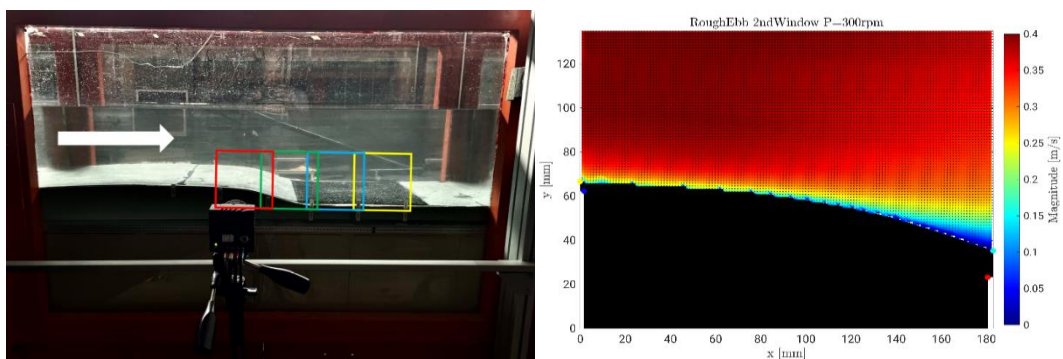
Fig. 1. Experimental configuration and visualization of PIV measurements. Left panel shows a photo of the experimental setup. The PIV camera points to the measuring area where different PIV windows are represented by colored rectangles. Right panel shows raw PIV data in terms of velocity magnitude and directions over the crest of the central dune for the largest forcing and bottom
