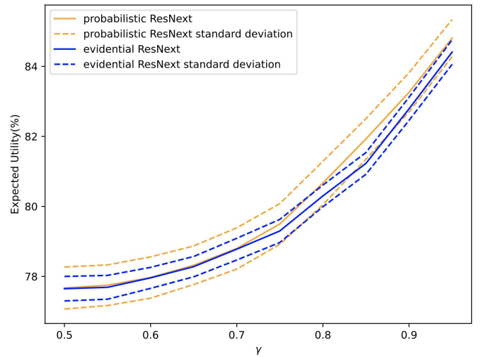
Figure 4. Expected Utility on CIFAR-100.
