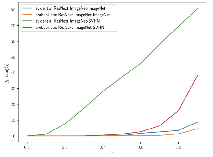
Figure 9. f_{\Omega} rate for OOD detection, ImageNet.
