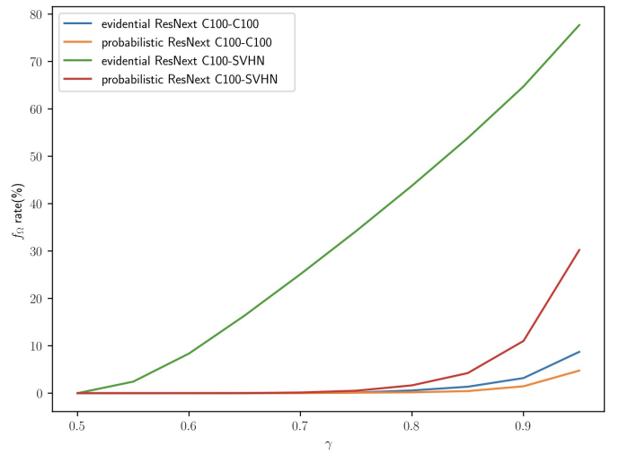
Figure 8. f_{\Omega} rate for OOD detection, CIFAR-100.
