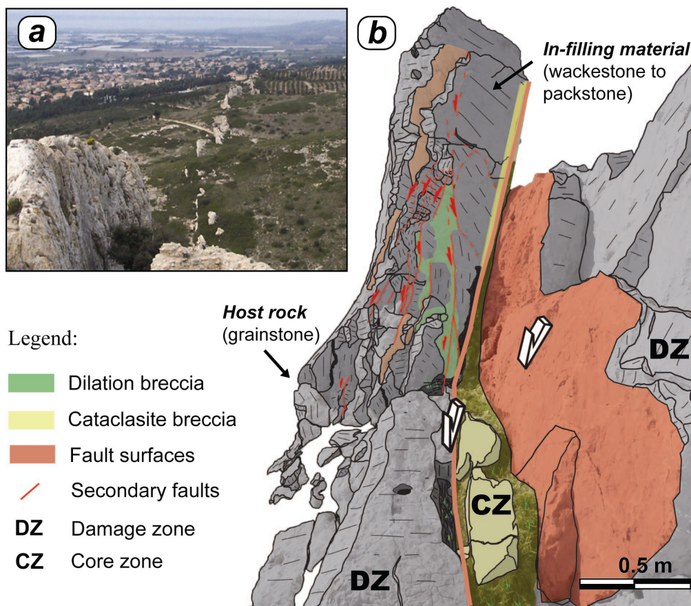
Figure 1 (a) Overview of the Castellans fault cropping out as a resistant relief along its entire length compared to the eroded porous host grainstone. The background shows the village of La Fare les Oliviers and the Etang de Berre. (b) Scheme of the studied Belvedere fault zone showing the compartmentalisation of the deformation.
