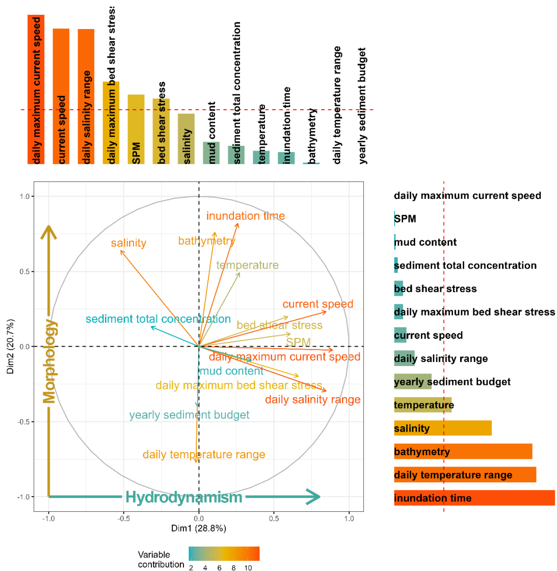
Figure 2 - Principal Components Analysis (PCA) variables correlation plot of the two main axes with the abiotic factors' contributions in bar plots for each axis. The colour of arrows and bars correspond to the contribution value of each variable. The red dotted line represents the mean contribution for all factors. The contribution of a variable to a given principal component is calculated as (\text{Variable} \cdot \cos^2 \cdot 100) / (\text{total } \cos^2 \text{ of the component}) .
