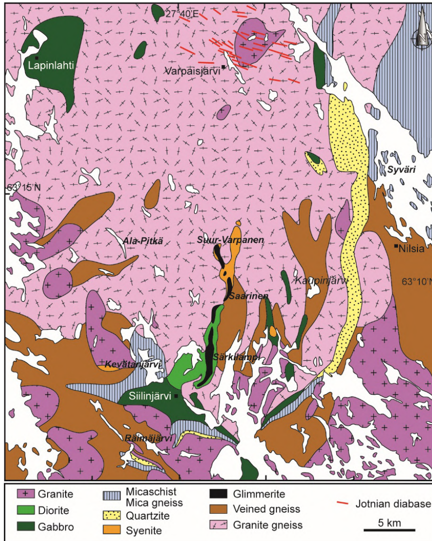
Figure 1.18. P-REE and carbonatite complex in Siilinjärvi, Finland (Pusstinen 1971)
