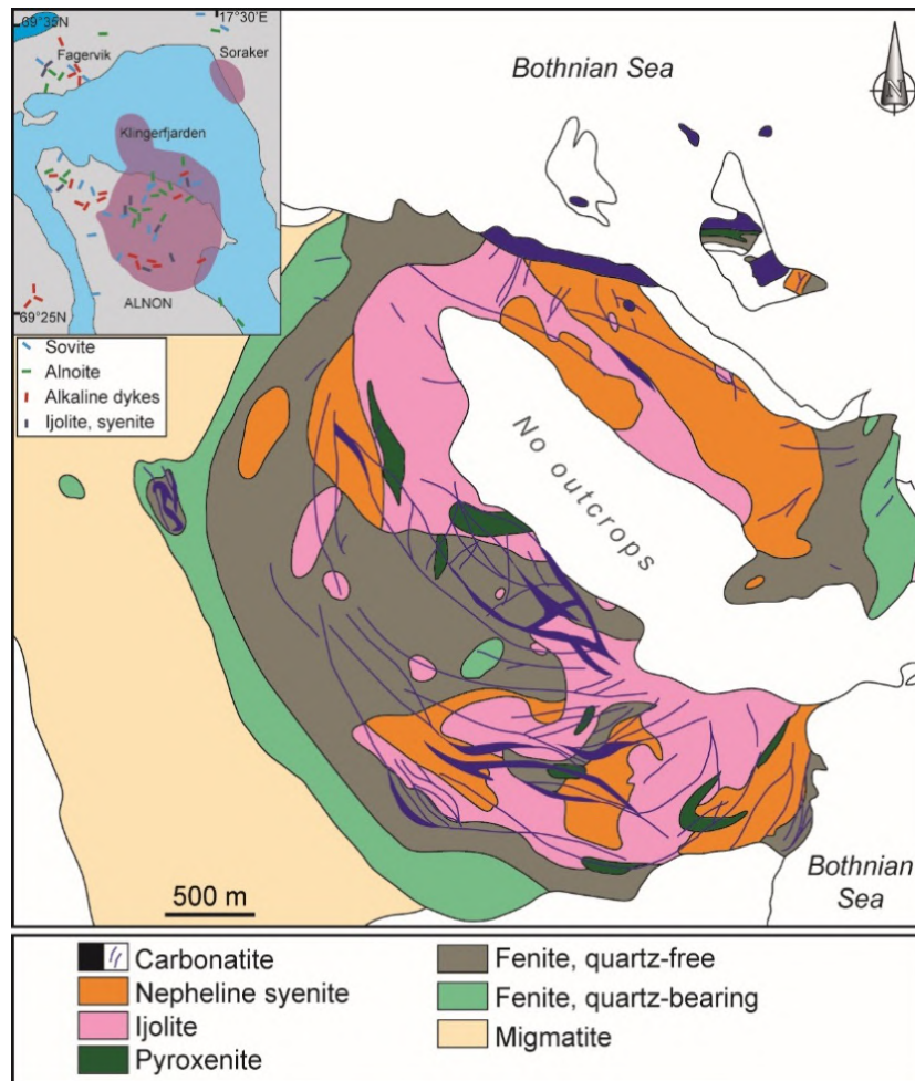
Figure 1.20. Nb-Zr-REE alkaline complex in Alnö (Sweden), modified from Vuorinen and Hålenius (2005)
