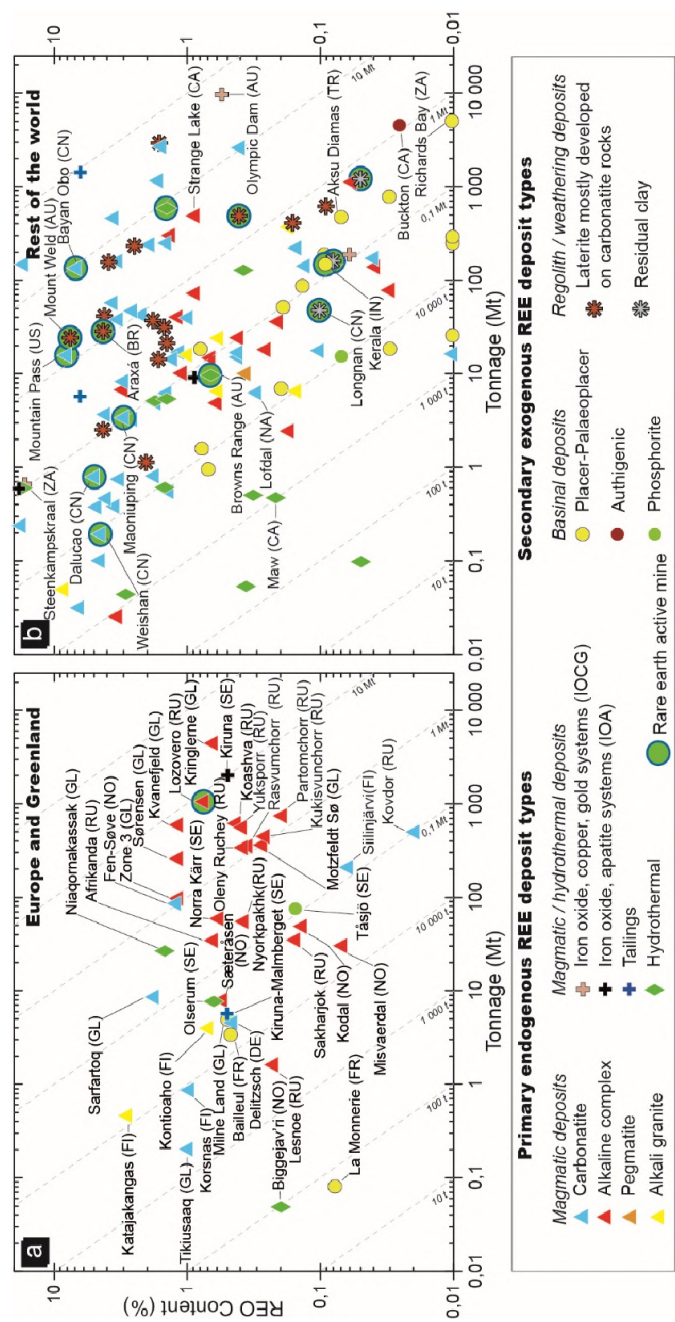
Figure 1.42. Grade/tonnage relationship for the different types of localized rare earth deposits
