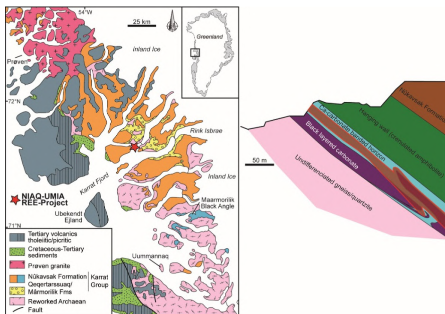
Figure 1.36. Deposits from the Paleoproterozoic at Karlat (NIAQ and UMIA) (Avannaa Resources 2010)
