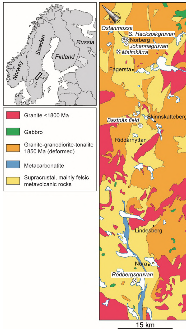
Figure 1.21. Bastnäs type Fe-REE-(Cu) skarns, Sweden (Holtstam and Andersson 2007)
