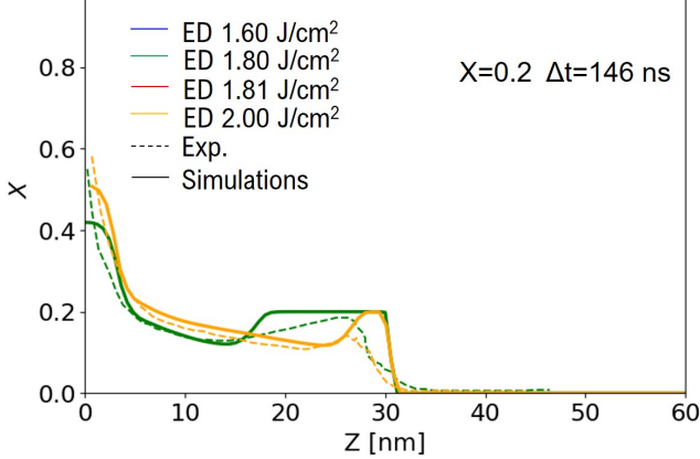
Figure 6: Schematics of the mono-dimensional model employed for laser annealing simulations on strained \text{Si}_{1-x}\text{Ge}_x samples (a), comparison between experimental and simulated MDs for a laser pulse of 146 ns (b)(c) and 160 ns (d)(e), experimental vs simulated germanium profile for X=0.2 (f) and X=0.4 (g) with \Delta t of 146 ns, the experimental profiles are re-drawn from Dagault et al. (2019, 2020). Cf. main text for definitions of original and calibrated models.
