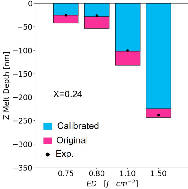
Figure 4: Schematics of the mono-dimensional model employed for simulating laser annealing on relaxed \text{Si}_{1-x}\text{Ge}_x samples (a), comparison between experimental and simulated MD for relaxed \text{Si}_{1-x}\text{Ge}_x samples with initial alloy fractions of 0.24 (b) and 0.58 (c). Cf. main text for definition of calibrated and original models
