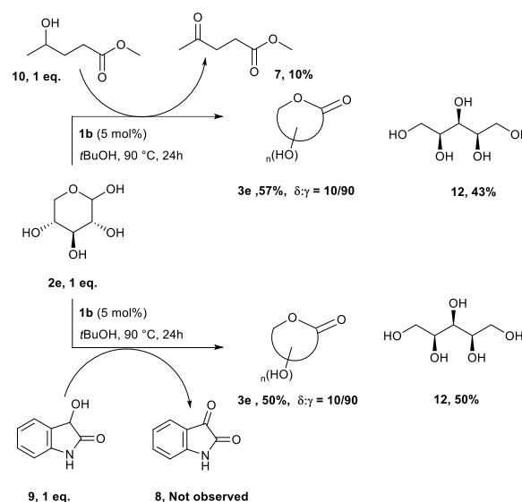
Scheme 4: Study of the reversibility of the process under the reaction conditions
