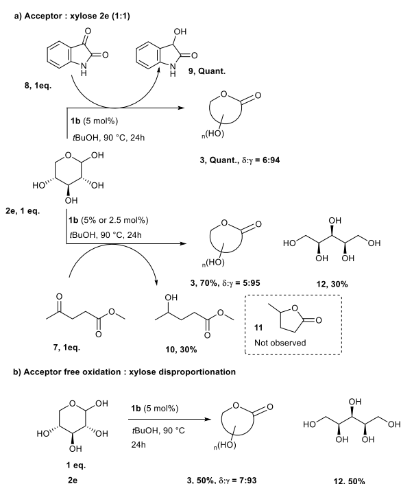
Scheme 4: Study of the reversibility of the process under the reaction conditions
