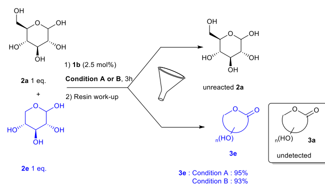
Scheme 2: Selective oxidation of xylose 2e in an equimolar mixture of glucose ( 2a ) and xylose ( 2b )
