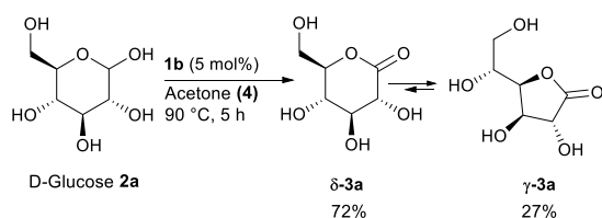
Scheme 1: Initial attempt on glucose oxidation with Knölker catalyst 1b . Yields of 3 were determined by 1 H NMR of the crude mixture (DMSO-d 6 ) using an internal standard.
