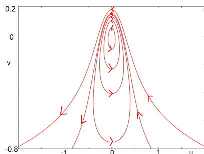
Figure 7. Solutions of the integrable Equation (13). The fixed point lies in the middle of limit cycles (nonlinear center). Above some threshold, solutions are no longer periodic but rather escape the vicinity of the stationary point. This illustrates the behavior of Figure 3: some canards exit to the left, while others exit to the right.
