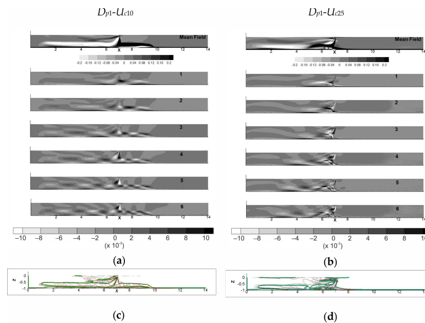
Figure 10. Mean solid phase velocity field and POD2C spatial dimensionless eigenfunctions \Phi_k(\vec{x}) obtained for the difference compared to the mean solid volume velocities ( u_s', w_s' ). To represent these eigenfunctions, it is necessary to calculate a pseudo-vector field equal to the rotation of the two-dimensional vector field. Dark colors represent positive values and clear colors represent negative values: (a) D_{p1-Uc10} ( M = 200 ); (b) D_{p1-Uc25} ( M = 140 ); outline obtained for the solid volume fraction velocities (solid line) superimposed to the four first eigenfunctions for (c) D_{p1-Uc10} and (d) for D_{p1-Uc25} .
