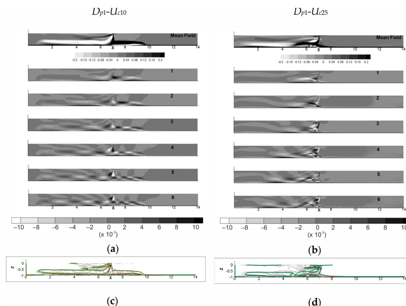
Figure 10. Mean solid phase velocity field and POD2C spatial dimensionless eigenfunctions \Phi_k(\vec{x}) obtained for the difference compared to the mean solid volume velocities ( u_s', w_s' ). To represent these eigenfunctions, it is necessary to calculate a pseudo-vector field equal to the rotation of the two-dimensional vector field. Dark colors represent positive values and clear colors represent negative values: (a) D_{p1-Uc10} ( M = 200 ); (b) D_{p1-Uc25} ( M = 140 ); outline obtained for the solid volume fraction velocities (solid line) superimposed to the four first eigenfunctions for (c) D_{p1-Uc10} and (d) for D_{p1-Uc25} .
