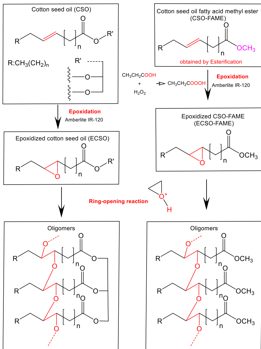
Figure 1. Reaction stages of esterification and epoxidation.
