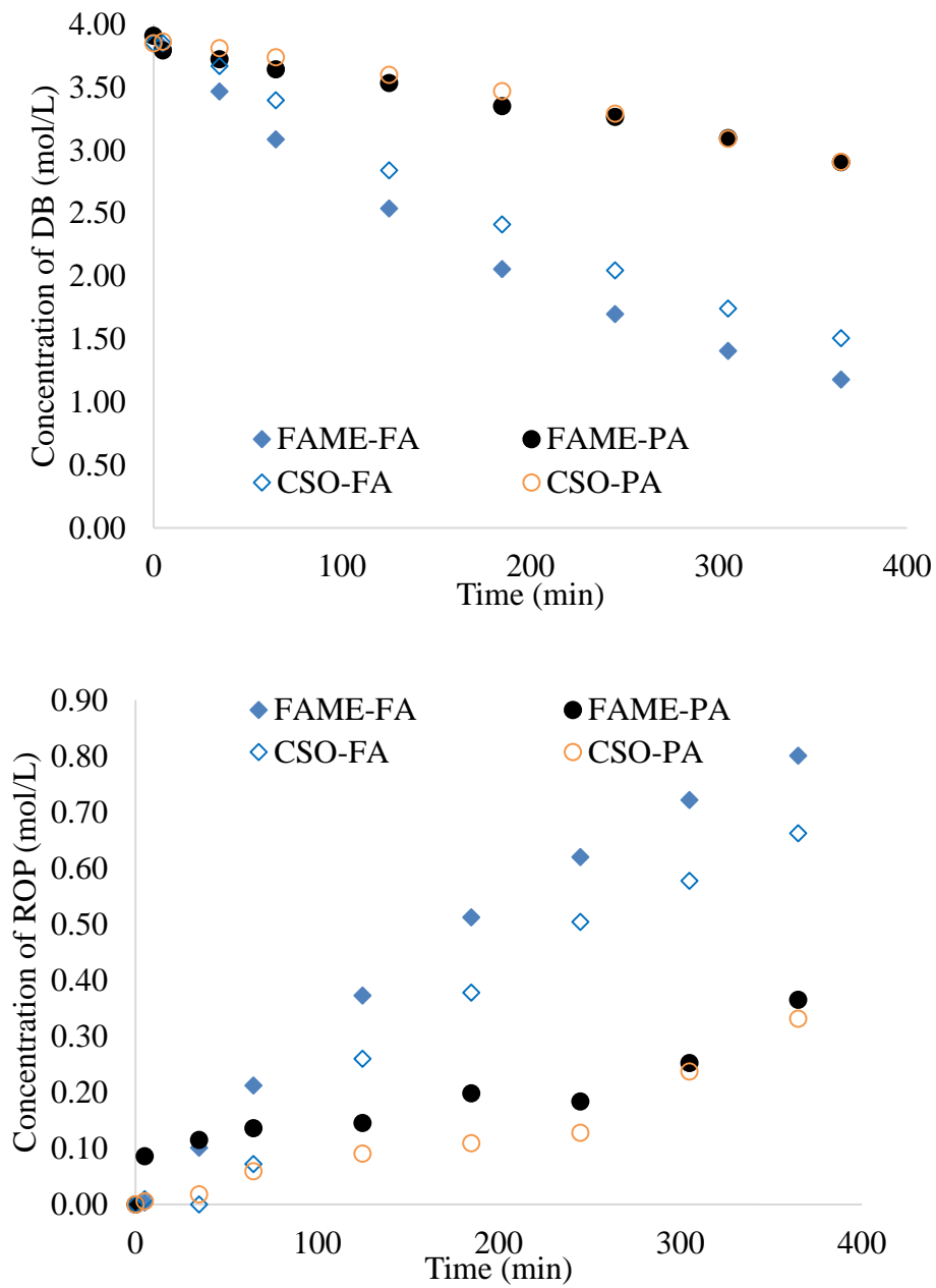
Figure 5. Effects of different acids on the epoxidation of CSO and CSO-FAME. (FA: formic acid; AA: acetic acid ; PA: propionic acid).
