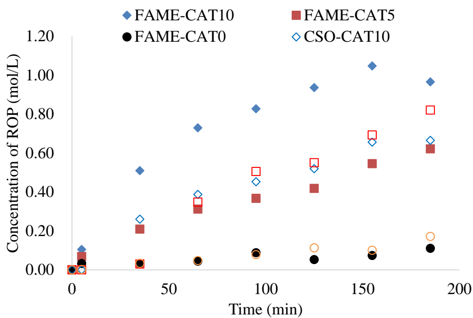
Figure 11. Effects of catalyst loading on the ring-opening products.
