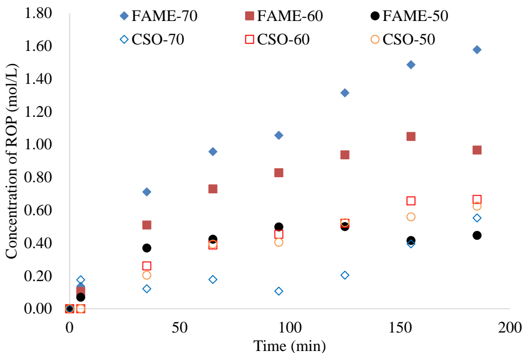
Figure 9. Effects of catalyst loading on the ring-opening products.
