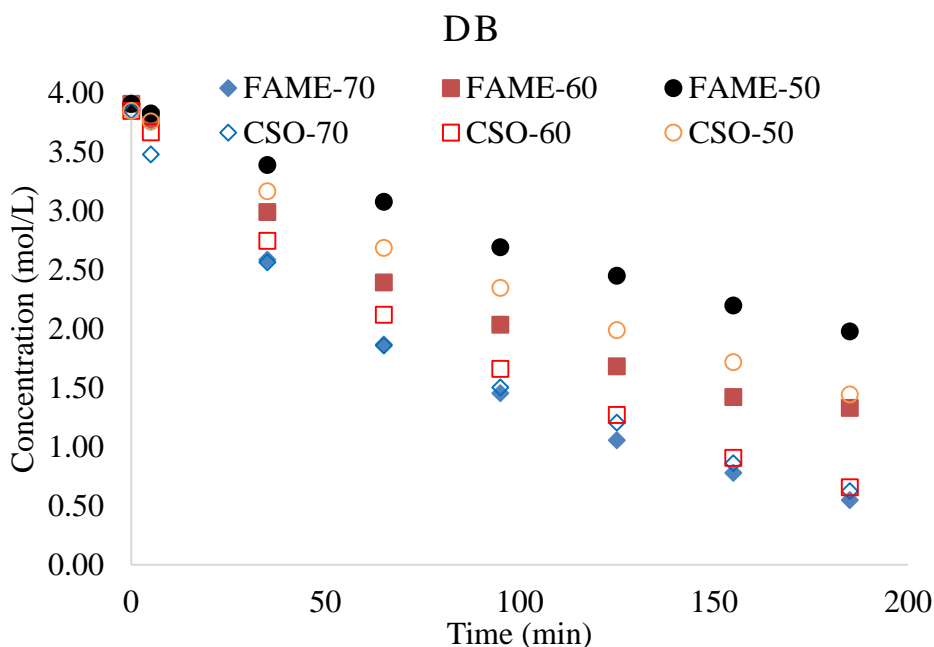
Figure 6. Effects of reaction temperature on the epoxidation of CSO and CSO-FAME by perpropionic acid (Runs 1, 2 and 3 from Tables 2 and 3).
