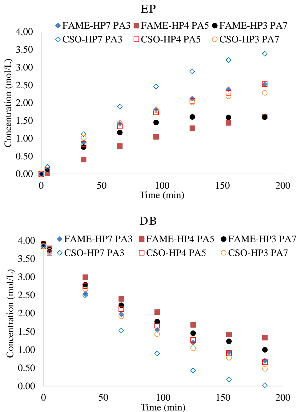
Figure 7. Effects of HP/PA ratio on the epoxidation of CSO and CSO-FAME by perpropionic acid (Runs 2, 5 and 6 in Tables 2 and 3).
