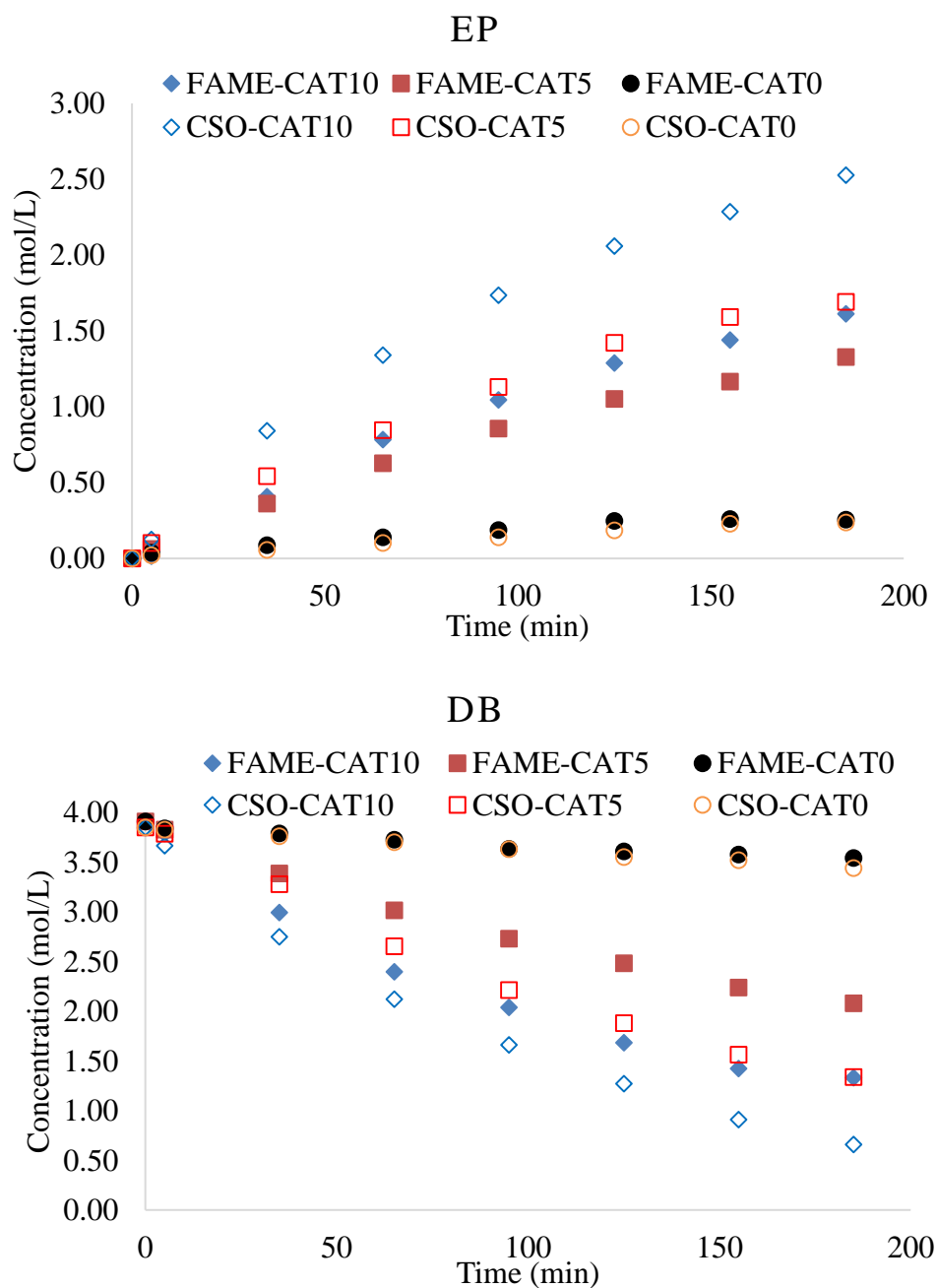
Figure 8. Effects of catalyst loading on the CSO and CSO-FAME.
