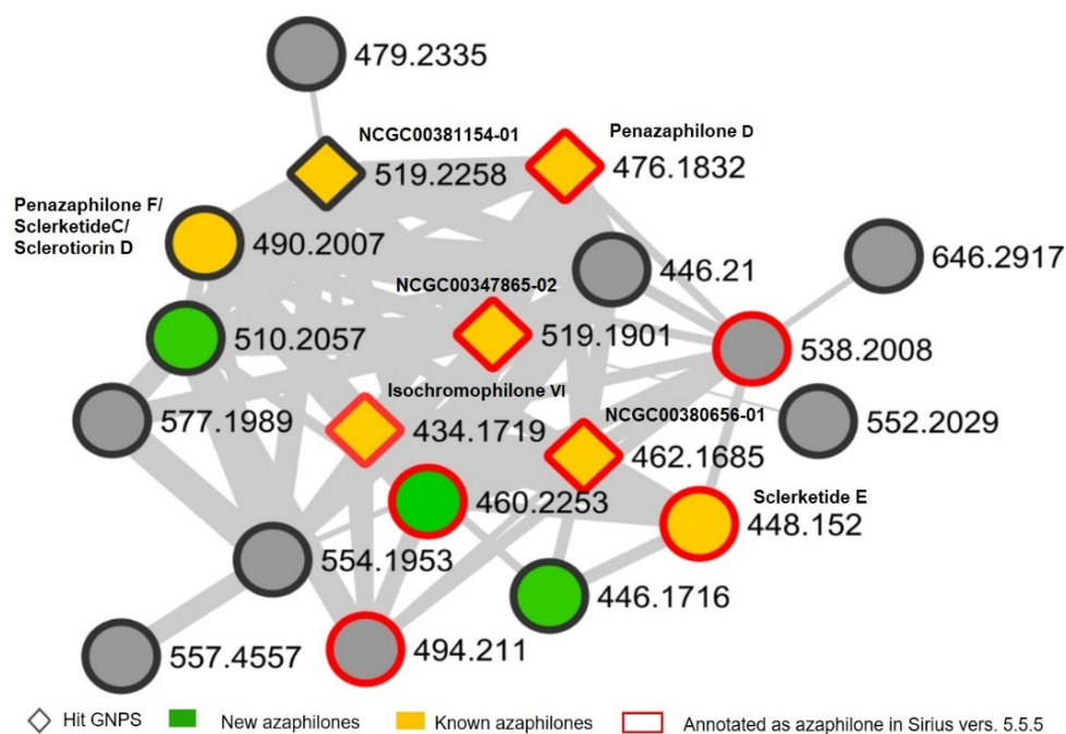
Figure 1. Cluster of azaphilones obtained from the molecular network of P. hirayamae crude extract and annotated by GNPS databases and Sirius vers. 5.5.5.
