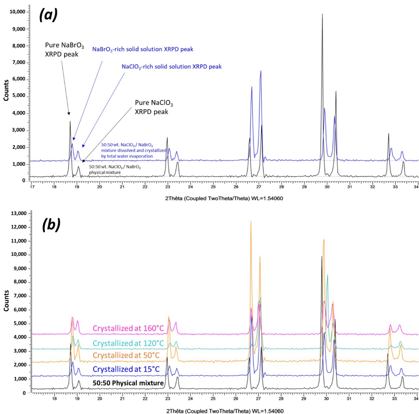
Figure 2. (a) XRPD pattern of powder sample (crystallized by slow evaporation under stirring from 50 wt.% \text{NaClO}_3/\text{NaBrO}_3 mixtures in aqueous solution) in comparison with pure \text{NaClO}_3 and \text{NaBrO}_3 (physical mixture). Two partial solid solutions exist: one \text{NaClO}_3 -rich solid solution (S.S.I) and one \text{NaBrO}_3 -rich solid solution (S.S.II). (b) XRPD patterns of powder samples crystallized by slow evaporation from 50 wt.% \text{NaClO}_3/\text{NaBrO}_3 mixtures in aqueous solution at different temperatures: RT, 15 °C, 50 °C, 120 °C, and 160 °C) confirmed that the miscibility gap is still present at elevated temperatures.
