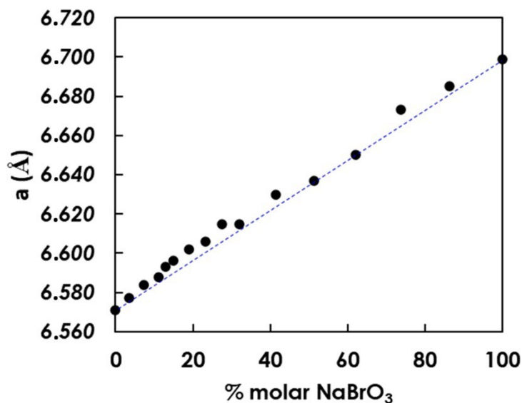
Figure 10. Crystallographic parameter a of the complete metastable solid solution \text{NaClO}_{3(x)}\text{BrO}_{3(1-x)} (molar fraction) prepared by spray-drying -using protocol 1 (precise values are reported in Table S1). A deviation from the Vegard law (apparent non-linearity) seems present for some compositions. The blue line is for guiding the eyes.
