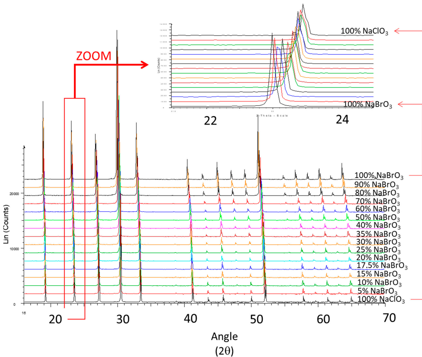
Figure 9. XRPD pattern versus composition of \text{NaClO}_3(x)\text{BrO}_3(1-x) (mass fraction) prepared by spray-drying-protocol 1-The inlet is a zoom on the second peak at ca. 23^\circ ( 2\theta scale \text{Cu K}\alpha ).
