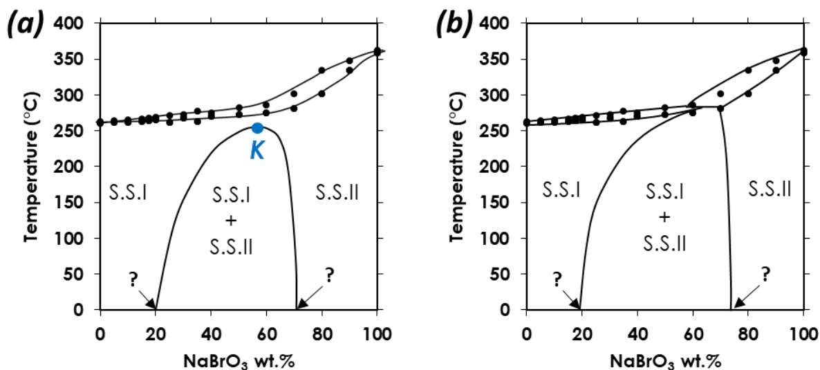
Figure 7. (a) Tentative homochiral binary phase diagram between NaClO 3 and NaBrO 3 showing a stable miscibility gap up to a critical point (K), above which a long period of diffusion time could succeed in mixing the two components in the full range of composition (i.e., from 0 to 100% NaBrO 3 ). Note that homochirality is supposed to appear to give left-handed or right-handed crystals only. (b) Tentative homochiral binary phase diagram between NaClO 3 and NaBrO 3 showing a stable miscibility gap that does not close up at elevated temperature but intersects the liquid-solid equilibria, implying a three-phase invariant (peritectic transition). Note: for both (a,b), filled circles correspond to experimental points determined by DSC (present work). Question marks, on x axis, reflect the difficulties to find the precise limits of the miscibility gap for stable equilibria.
