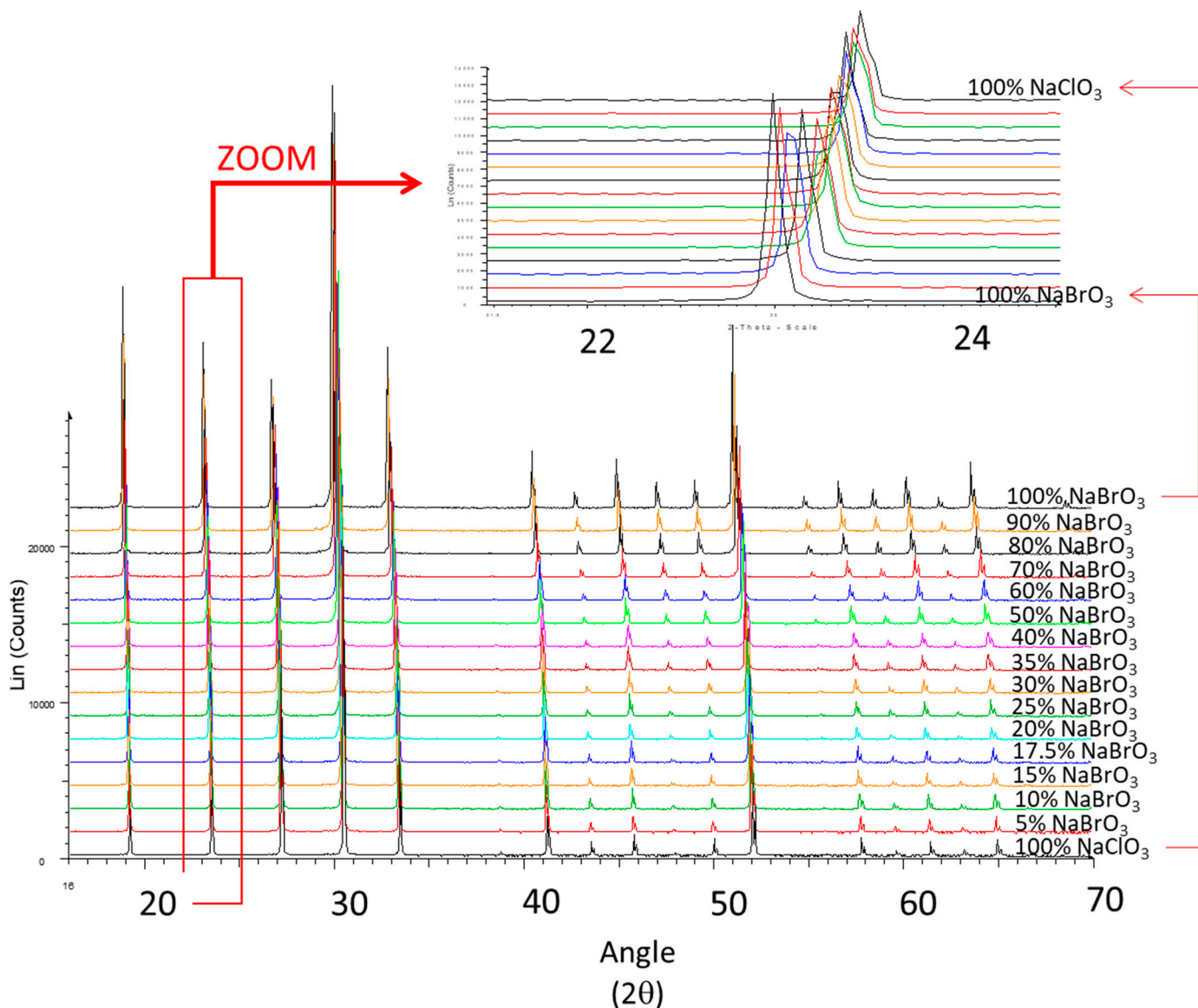
Figure 9. XRPD pattern versus composition of \text{NaClO}_{3(x)}\text{BrO}_{3(1-x)} (mass fraction) prepared by spray-drying-protocol 1-The inlet is a zoom on the second peak at ca. 23^\circ ( 2\theta scale \text{Cu K}\alpha ).
