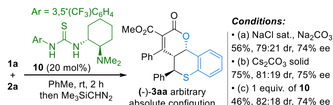
Scheme 4. An enantioselective domino VMAC reaction.
