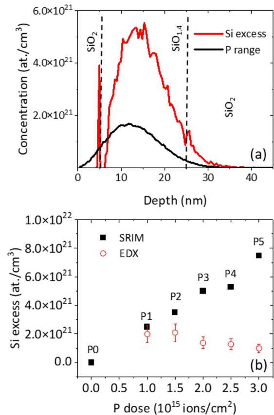
Fig. 6 (a) Profiles of the P range (black line) and Si excess (red line) for sample P4, calculated by SRIM. (b) Evolution with the dose of Si supersaturation remaining in the matrix after annealing in the NC region as measured by STEM-EDX (open circles) compared to the Si excess in the NC region associated with the recoiling atoms, as predicted by SRIM after the P implantation (black squares).
