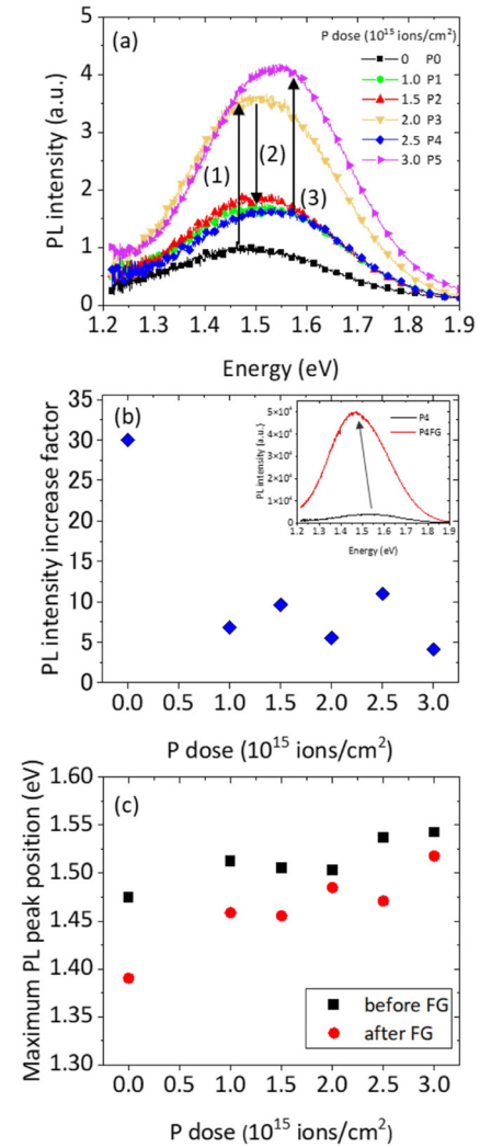
Fig. 7 (a) PL spectra of the of the undoped and doped samples implanted with various P doses prior to FG annealing (excitation with a xenon lamp filtered at 325 nm). (b) Ratio of the PL intensity (measured at the peak maximum) before and after FG annealing (ratio = PL_{FG}/PL ). The inset shows the PL spectra of P4 before (black) and after (red) FG annealing. (c) Position of the PL peak before and after FG annealing.
