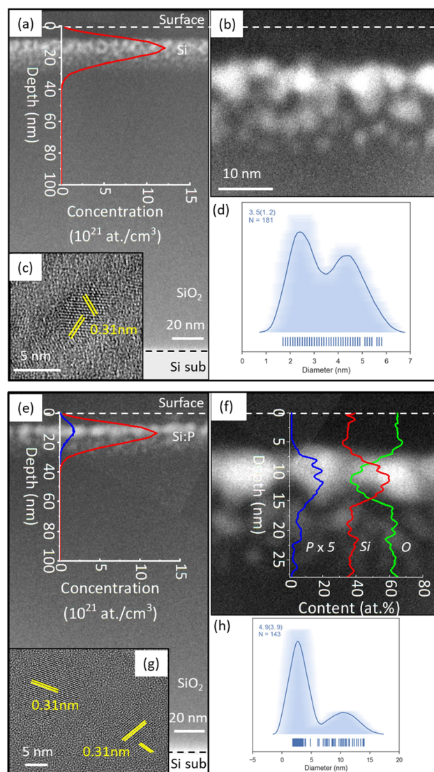
Fig. 1 (a) and (e) EFTM cross-sectional images displaying the spatial distribution of undoped (P0) and doped (P4FG) SiNCs with associated SRIM profiles for Si (red line) and P (blue line). Zoom-in on the NC region for (b) the undoped and (f) doped samples, with associated EDX profiles for Si (red line), O (green line) and P (blue line). (c) and (g) HREM images of a large SiNC in the (110) zone axis. NC average shifted histograms (ASH) 25 showing the bimodal size distributions for the undoped (d) and doped (h) samples.
