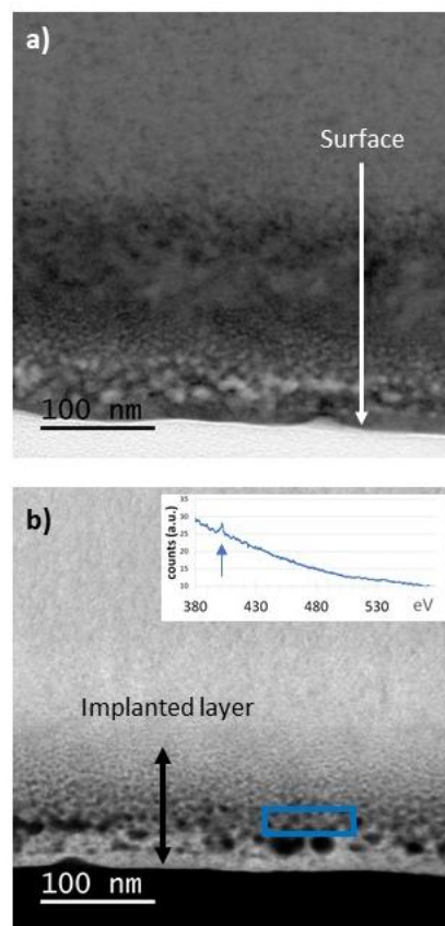
Figure2: Cross sectional view of the recrystallized CuSn8 alloy implanted with nitrogen with the surface located at the bottom, a) STEM-BF image, b) STEM-HAADF image with inset the EELS spectra recorded in the implanted layer showing a peak at the N-K edge
