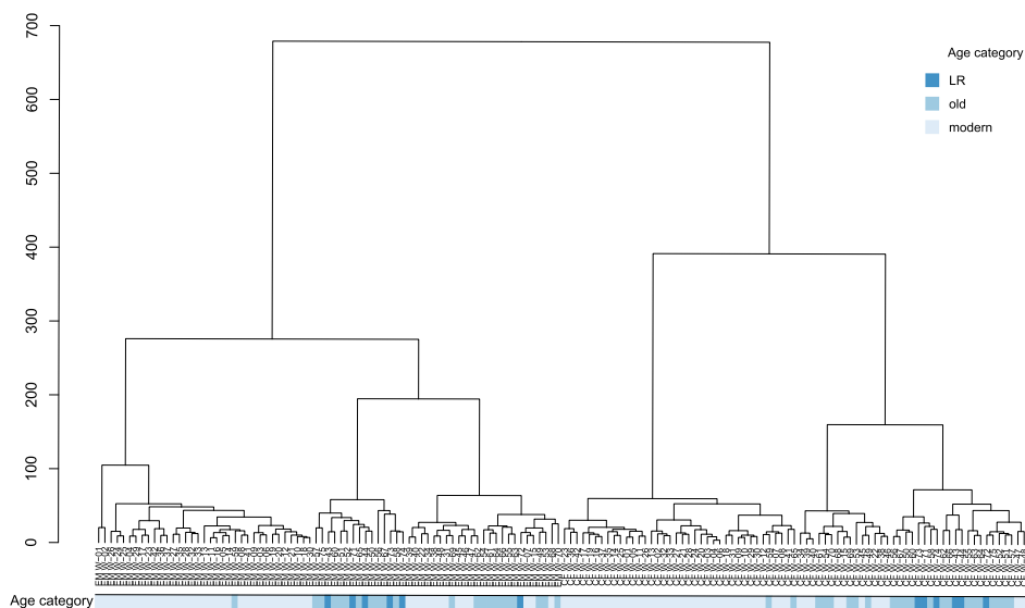
Fig. 3. Clustering of the 75 varieties cultivated at Clermont–Ferrand (CF) and Estrées–Mons (EM) based on the mean of the two replicates for each location. Manhattan distance was used to calculate dissimilarities among varieties for grain hardness, thousand–kernel weight, protein composition, polymer characteristics and technological properties. The Ward D agglomeration method was used for clustering. The shaded horizontal bar indicates the age category of each variety.
