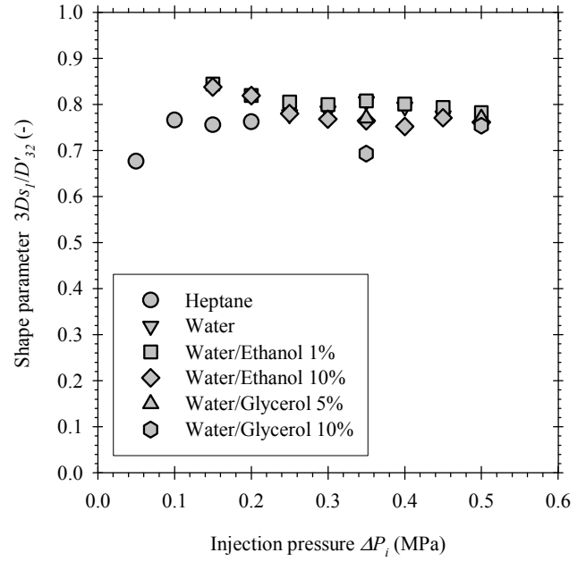
Fig. 12: Relationship between the ratio 3D_{S_l}/D'_{32} and the injection pressure (all fluids).
