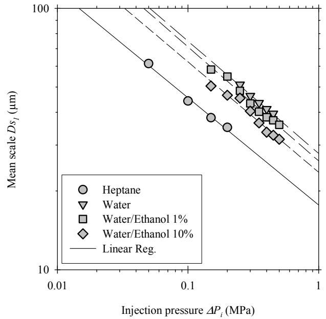
Fig. 10: Evolution of the mean scale Ds_1 as a function of the injection pressure (several fluids).
