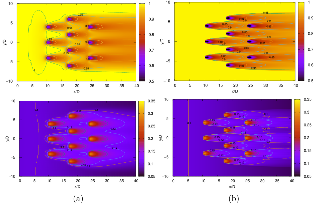
FIGURE 6 – Numerical (a) and empirical (b) contour showing the normalized velocity (top) and the turbulence intensity (bottom) along the lateral plane.
