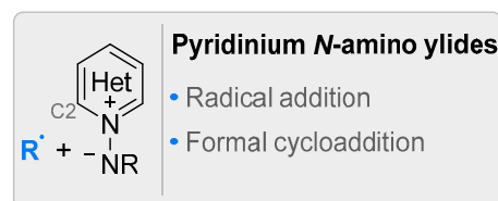
Figure 6. Radical-based transformations of pyridinium N -amino ylides.
