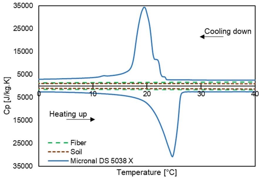
Figure 13: Evolution of the raw materials specific heat capacity as function of temperature.
