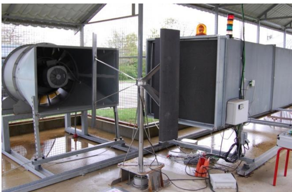
Fig 2. Experimental wind tunnel
