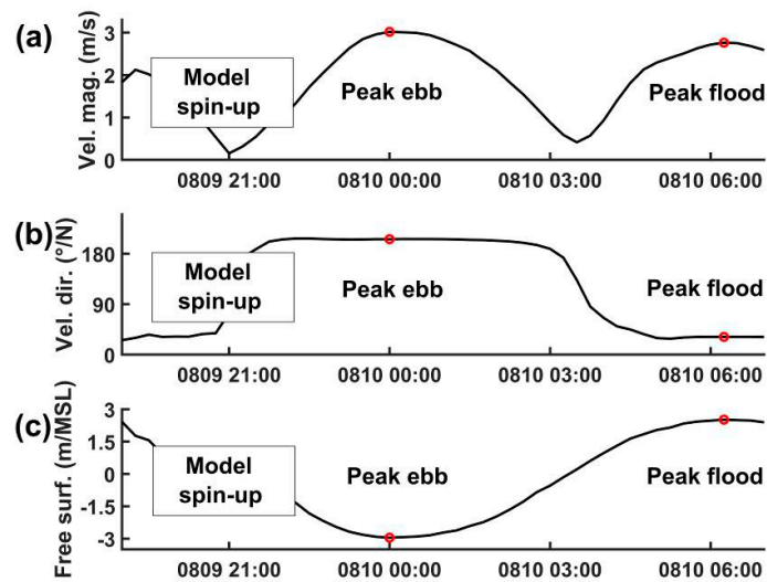
Figure 2. Time-series of (a) depth-averaged velocity magnitude, (b) depth-averaged velocity direction, and (c) free surface elevation extracted from the Telemac3D model (simulation without turbine) in the center of the fence ( 49^{\circ}42.300' N ; 2^{\circ}6.180' W ). The red circles show times of peak ebb and flood retained to assess the array efficiency.
