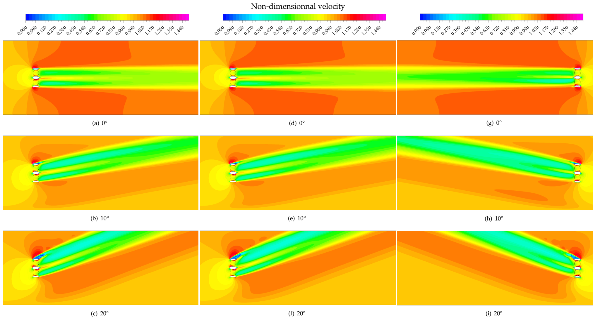
Figure 11. Flow around a single turbine: Non-dimensional velocity ( U_a = U/U_\infty ) field for U_\infty = 1.5 \text{ m} \cdot \text{s}^{-1} , (a–c), U_\infty = 3.0 \text{ m} \cdot \text{s}^{-1} (d–f), and U_\infty = -3.0 \text{ m} \cdot \text{s}^{-1} , (g–i).
