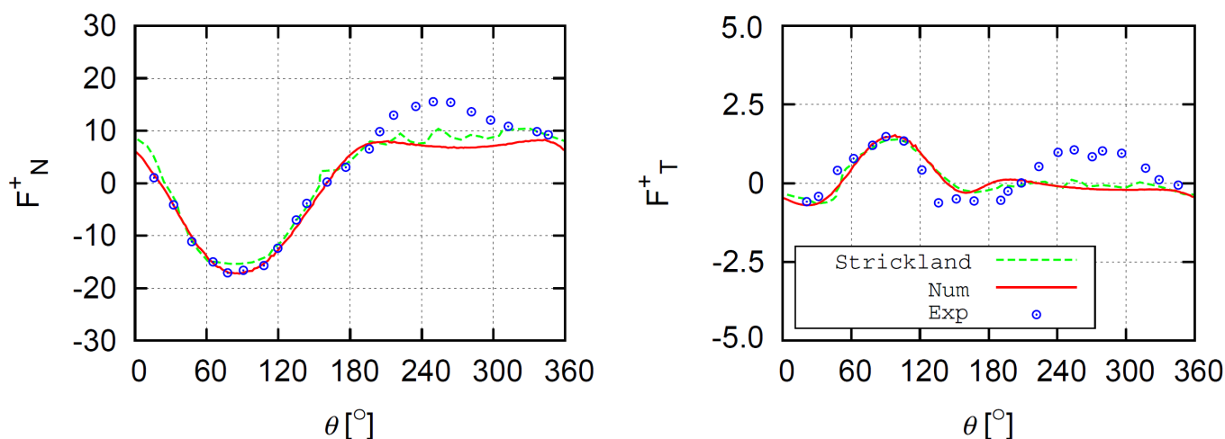
Figure 3. Normal (left) and tangential (right) forces in function of the azimuthal position \theta , comparison between the experience of Strickland for three blades and the numerical results of Nguyen et al. [2].
