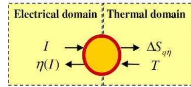
Fig. 7 Energetic conversion from electrical to thermal domain
