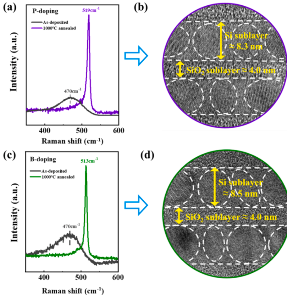
Fig. 1. (a) Raman spectra and (b) cross-sectional high-resolution TEM image of annealed P-doped Si NCs/SiO 2 multilayers; (c) Raman spectra and (d) cross-sectional high-resolution TEM image of annealed B-doped Si NCs/SiO 2 multilayers. The Raman spectra of as-deposited samples are also plotted for comparison.
