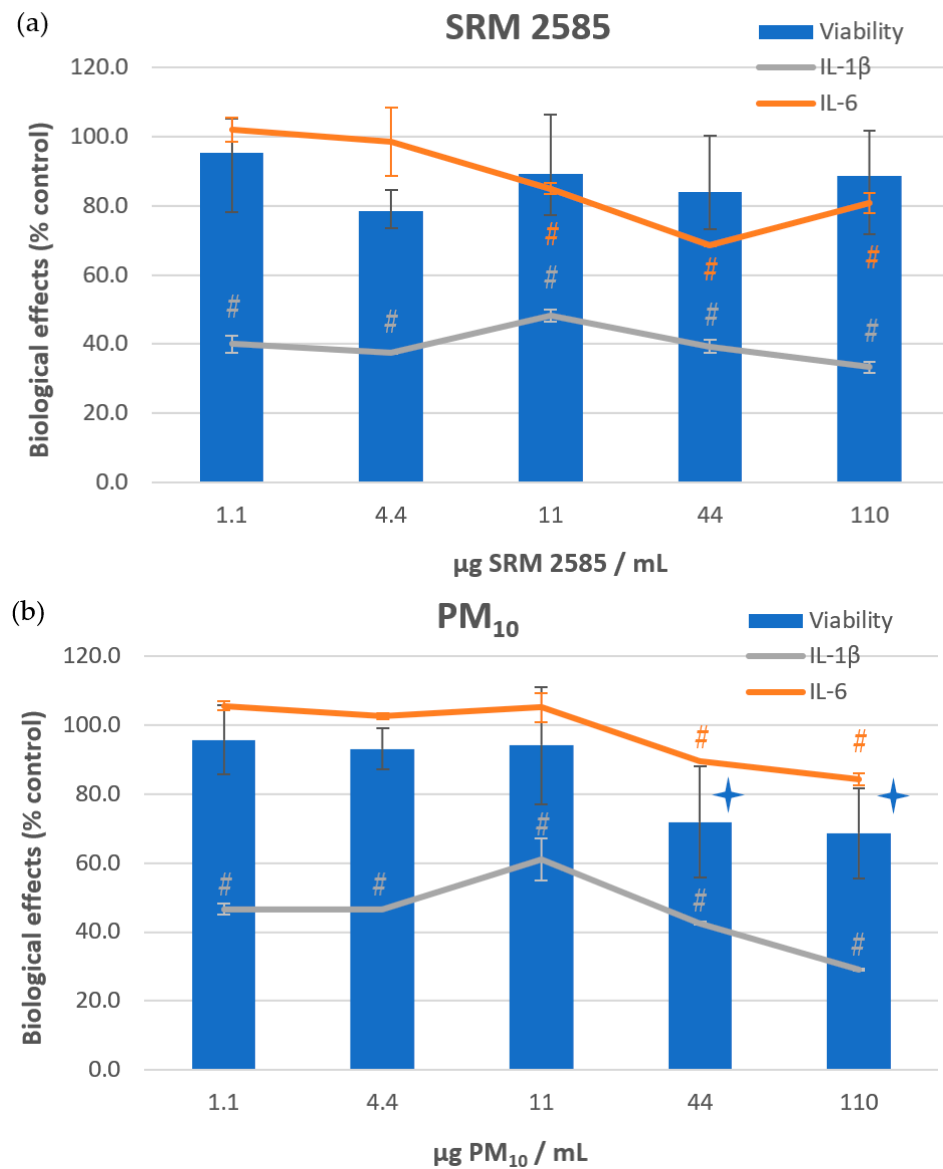
Figure 4. Biological effects measured on NHBE cells after 72 h exposure to either (a) SRM ® 2585 or (b) PM 10 fraction. Viability and cytokine production (IL-6, IL-1 \beta and TNF- \alpha ) were evaluated. Each condition was tested in two independent experiments, in triplicate for viability and in duplicate for cytokine production. Results are expressed relative to negative control. Student's test was performed on raw data. Significant reduction of NHBE viability (* \star ) or of cytokine excretion (#) ( p \leq 0.05 ).
