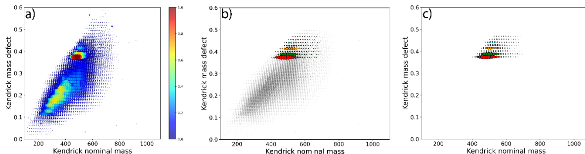
Figure S 2: a) Kendrick's diagram with all species, b) Kendrick's diagram with extracted series stacked on the previous plot, c) Kendrick's diagram with only the extracted series.
