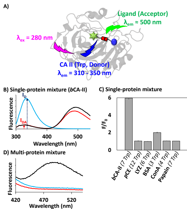
Figure 4. Analysis of Trp-FRET experiments. A) iFRET principle; B) Fluorescence emission spectra of a solution of bCA-II (2 \mu\text{M} ) in the absence (in blue), or in the presence of Z-3ah (2 \mu\text{M} in red, 4 \mu\text{M} in black), upon an excitation at 280 nm, in PB pH 7.4; C) Relative fluorescence intensity observed at 495 nm of a solution of Z-3ah (1 \mu\text{M} ) in the presence of various proteins (2.5 \mu\text{M} ), upon an excitation at 280 nm, in PB pH 7.4; and D) fluorescence emission of Z-3ah (1 \mu\text{M} ) in a solution containing five Z-3ah non-target proteins (PCE, LYZ, BSA, ConA, papain, 2.5 \mu\text{M} each) in the absence (in blue) or in the presence of bCA-II (2.5 \mu\text{M} , without ATZ in black; or with 100 \mu\text{M} ATZ in red), upon an excitation at 280 nm, in PB pH 7.4.
