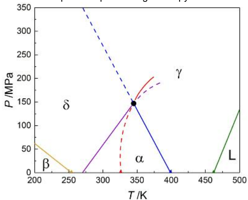
Pressure-temperature phase diagram of pyrazinamide
